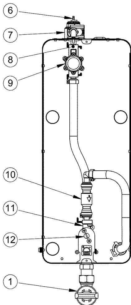
TOP VIEW COVER REMOVED
