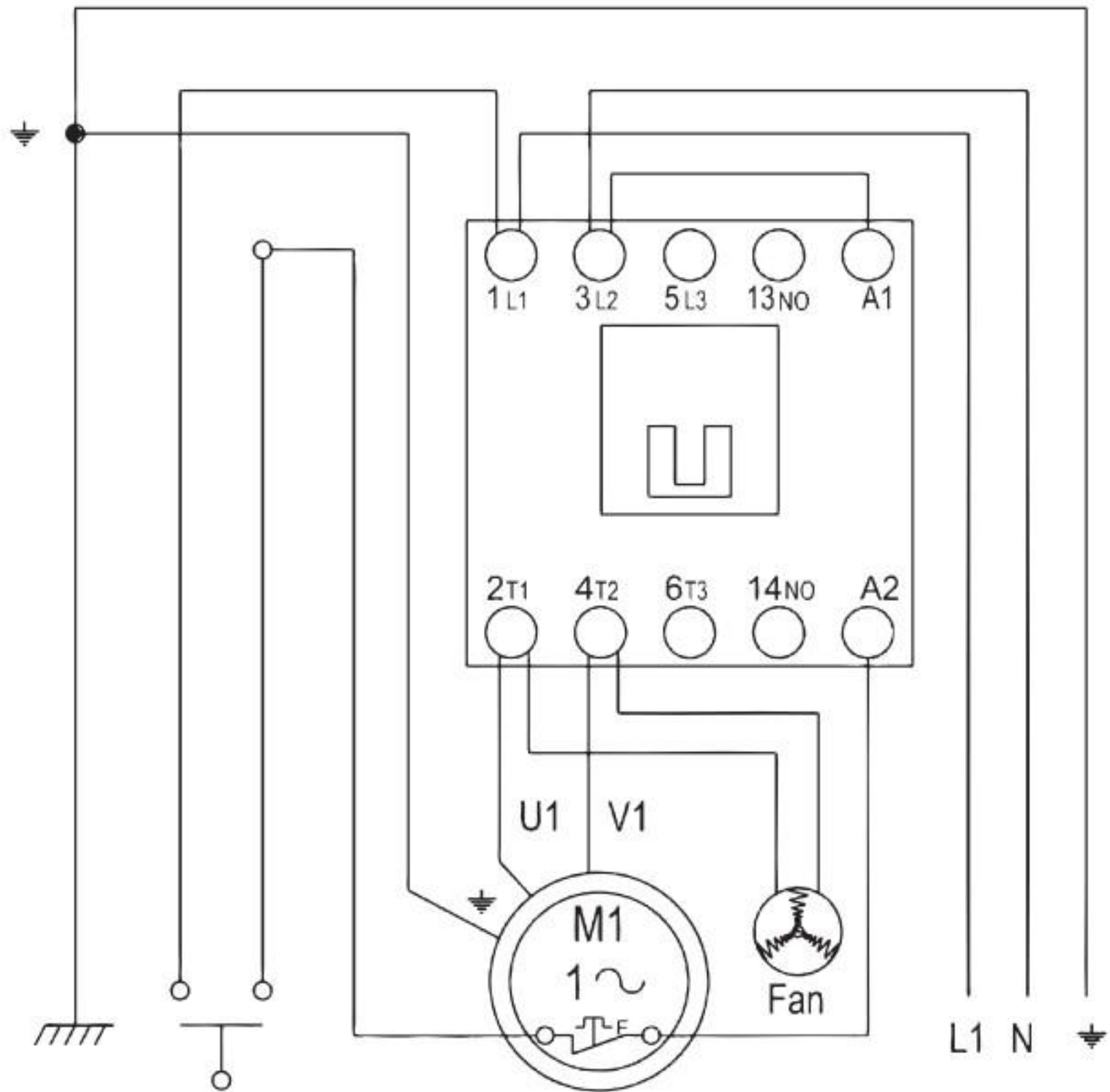
Motor with internal thermo protection
