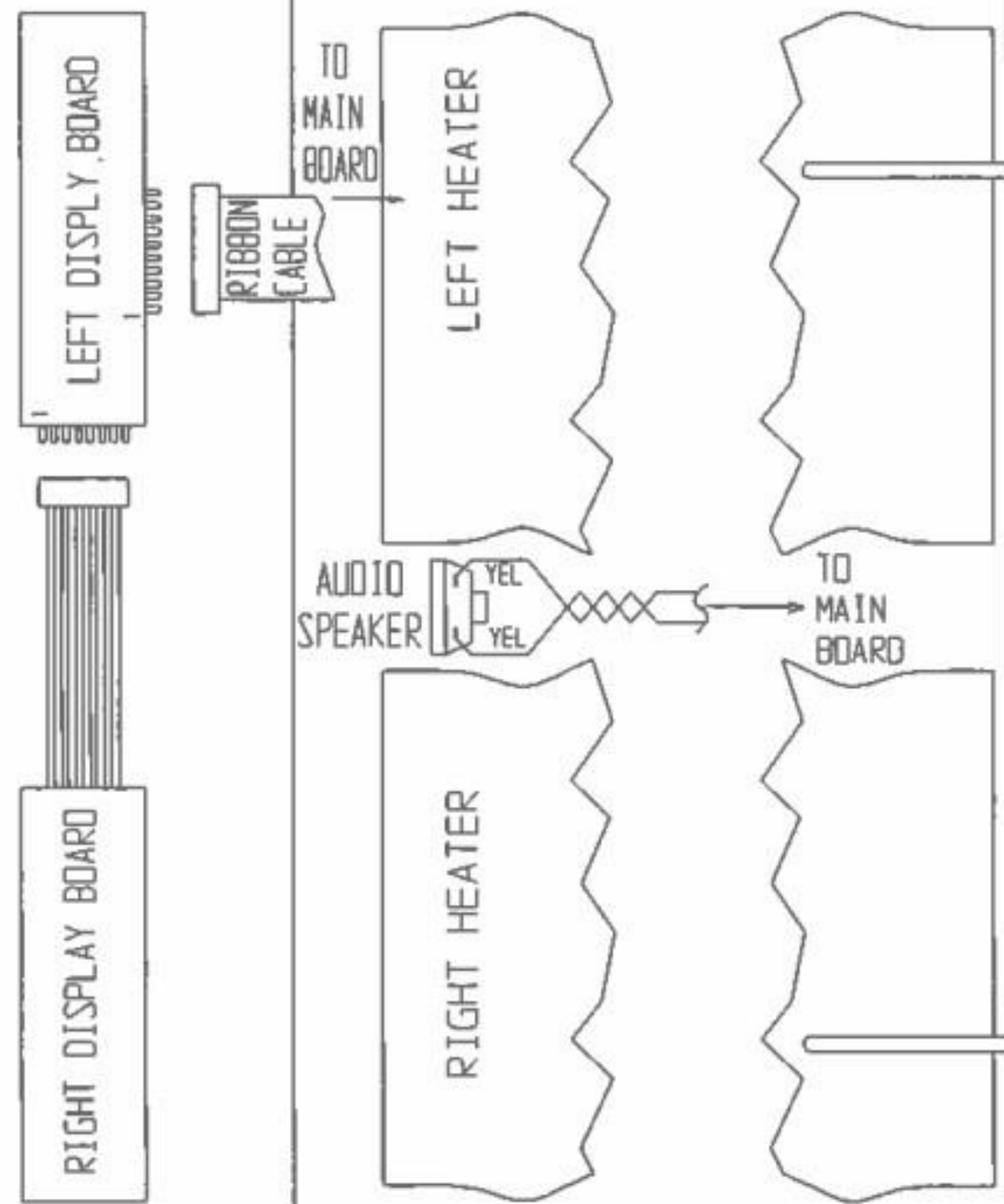
NO.424 DUAL CHAMBER TOASTER WIRING DIAGRAM 424-143, REV. -A
