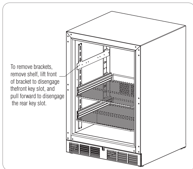
Figure 5. Sliding Shelf Mounting Brackets
