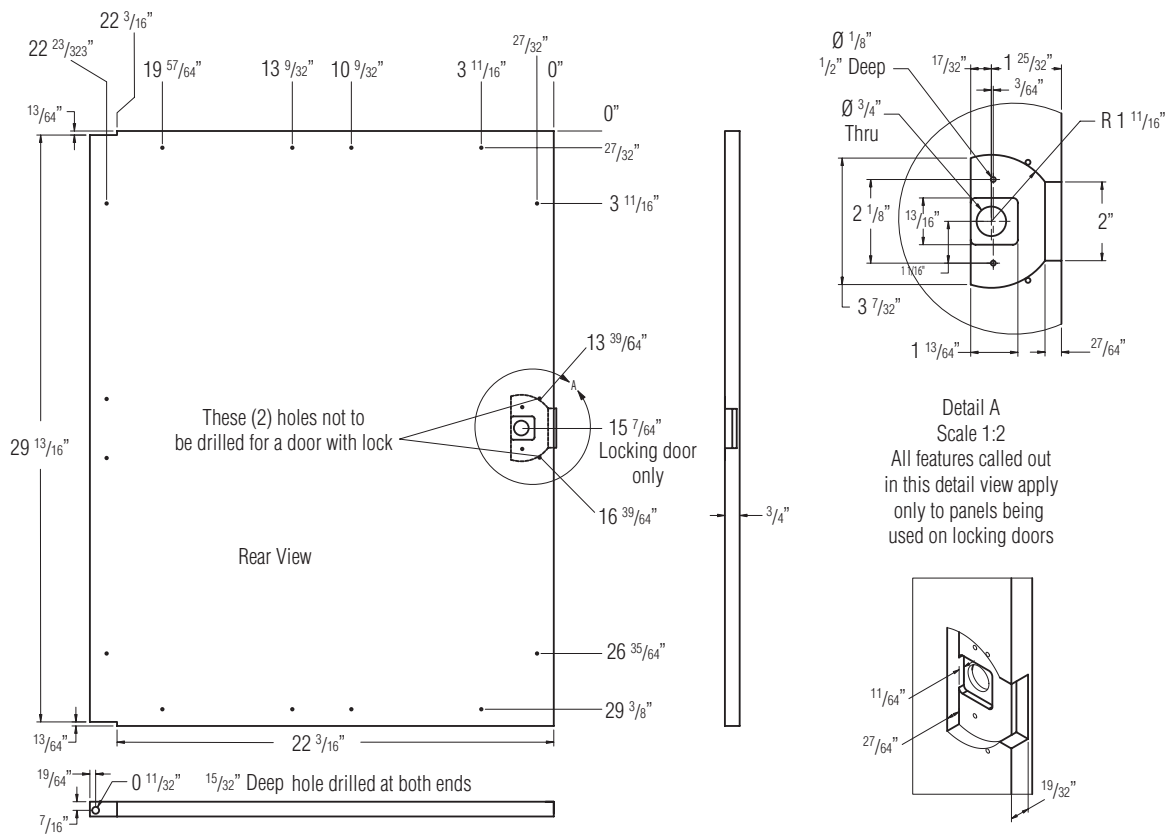
Figure 8. Solid Wood Overlay Door Panel
