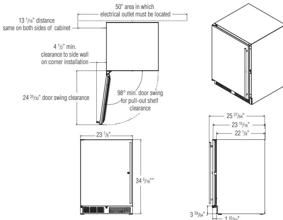
Figure 1. Dimensions
