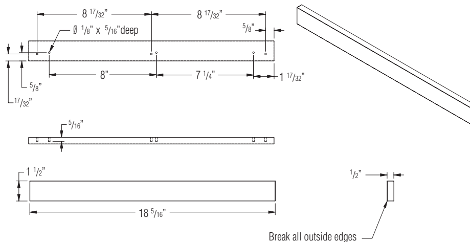
Figure 9. Wooden Wine Rack Trim
