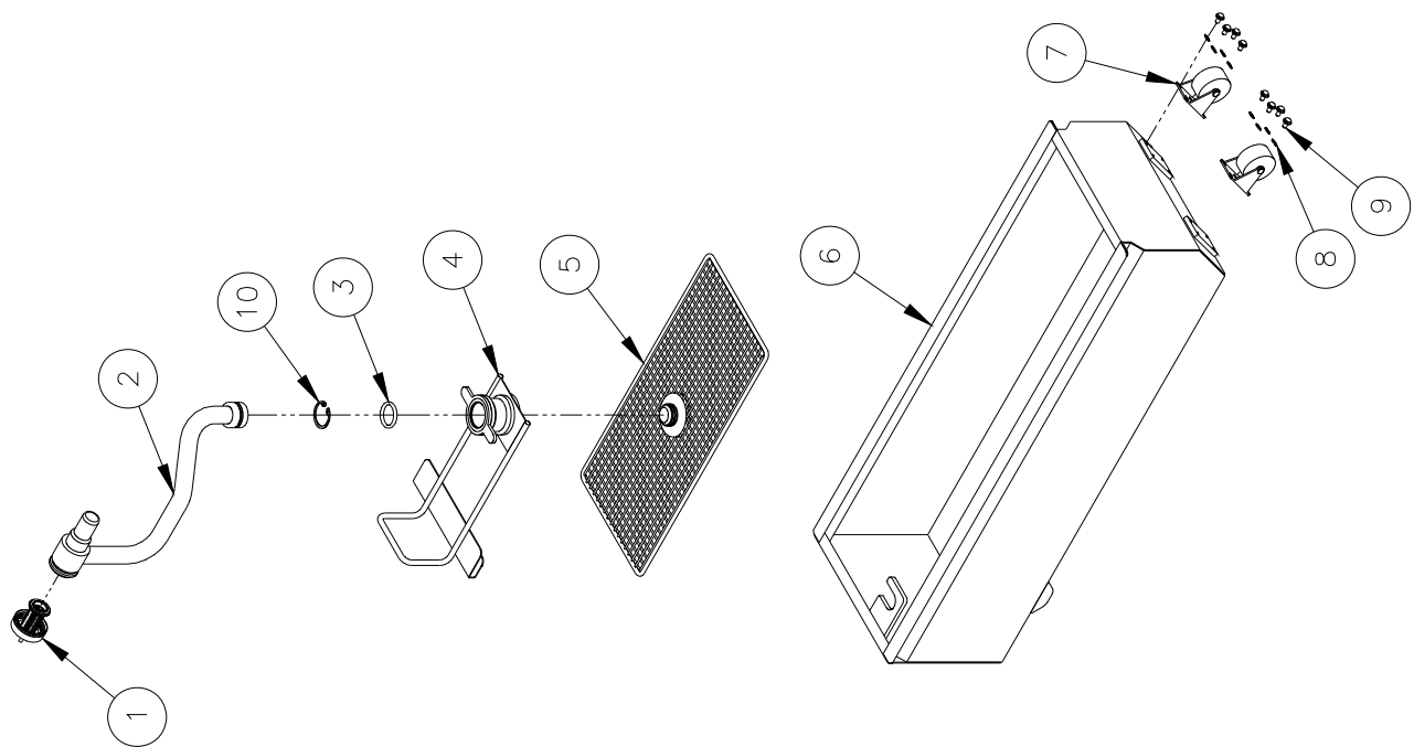
SFSG FILTER DRAWER (SOLOFILTER)
