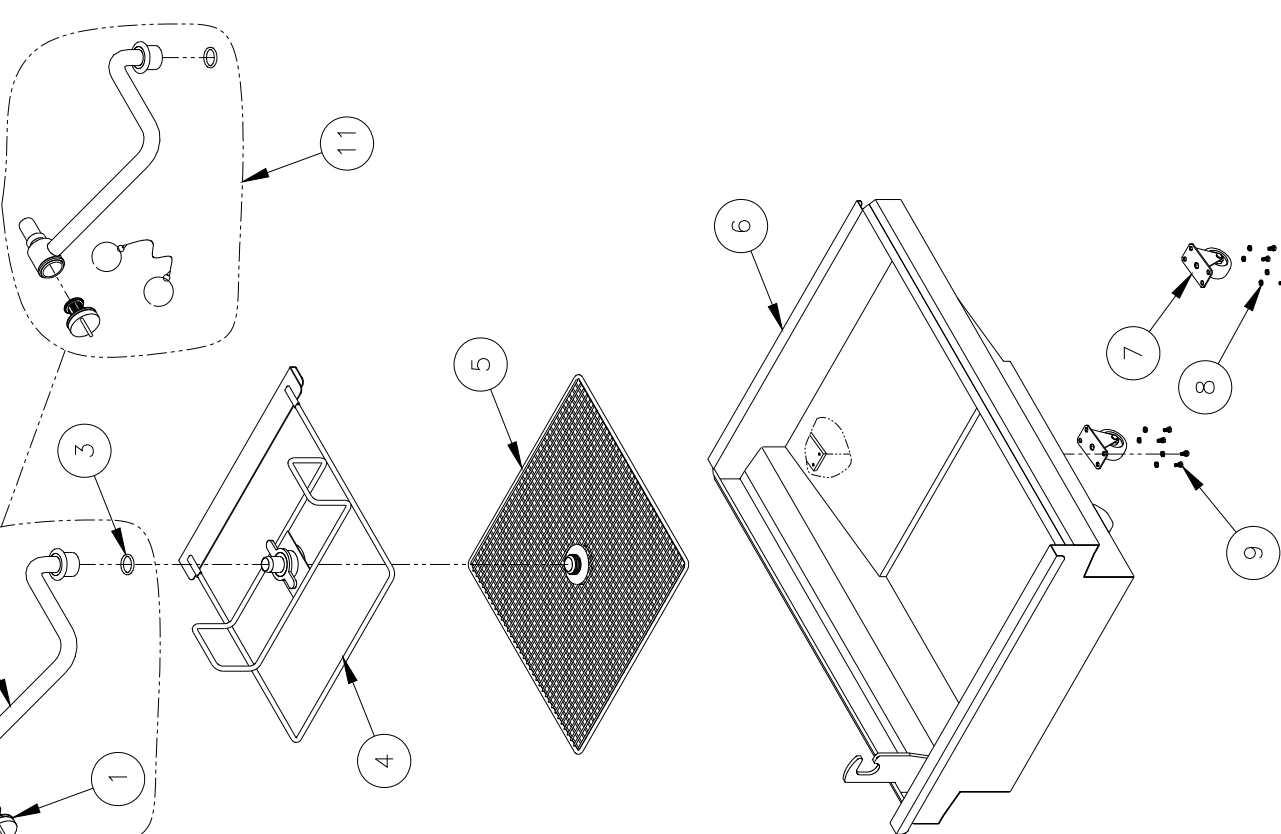
SG FILTER DRAWER AFTER 3/26/04
