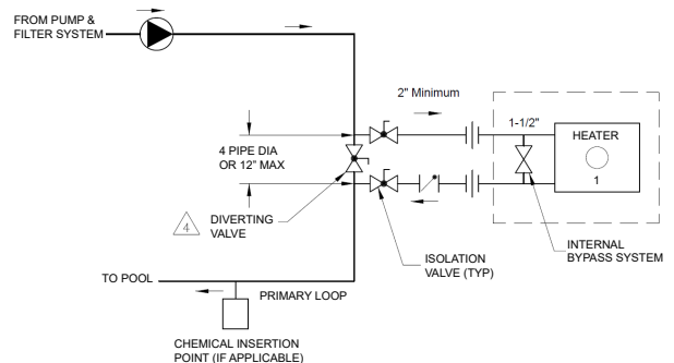
Figure 14. Piping Diagram
