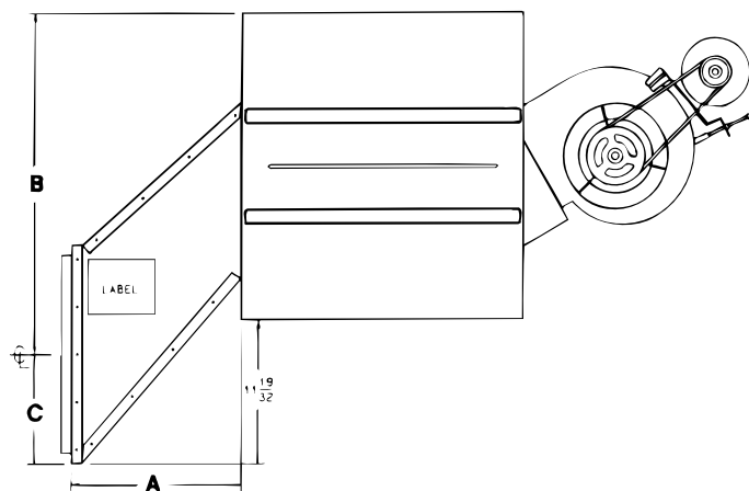
Figure 2 - Side View of Heater and Polytube Adapter, Option CD6, with Adapter Outlet Below the Heater Discharge
