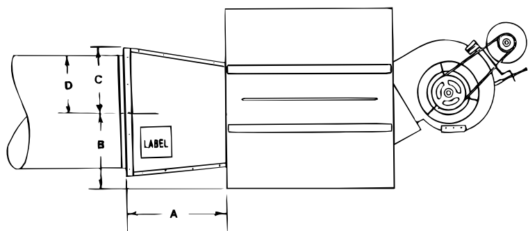
Figure 4 - Side View of Heater and Polytube Adapter, Option CD11
