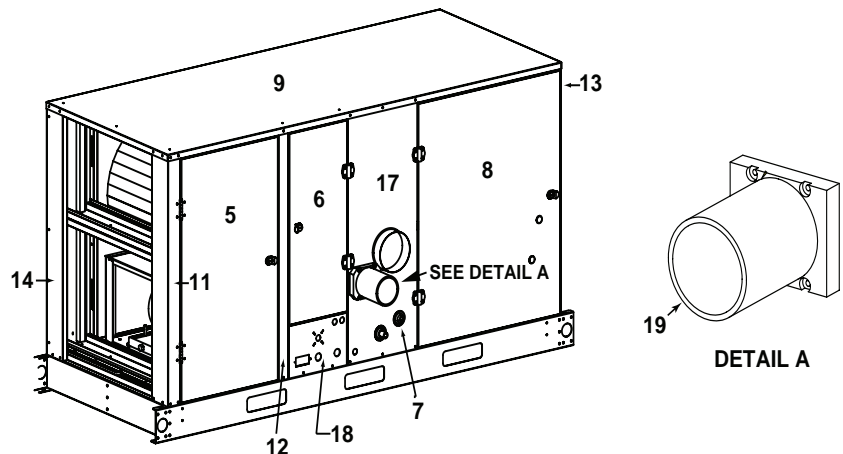
Figure 45. Cabinet Components—Indoor Model SHH (Refer to Table 67)
