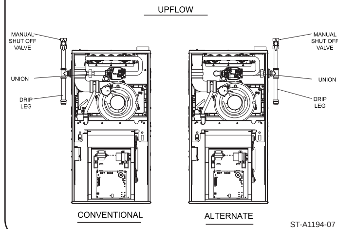
FIGURE 2 BURNER COMPARTMENT - SHOWING LOCATION OF GAS CONTROLS
