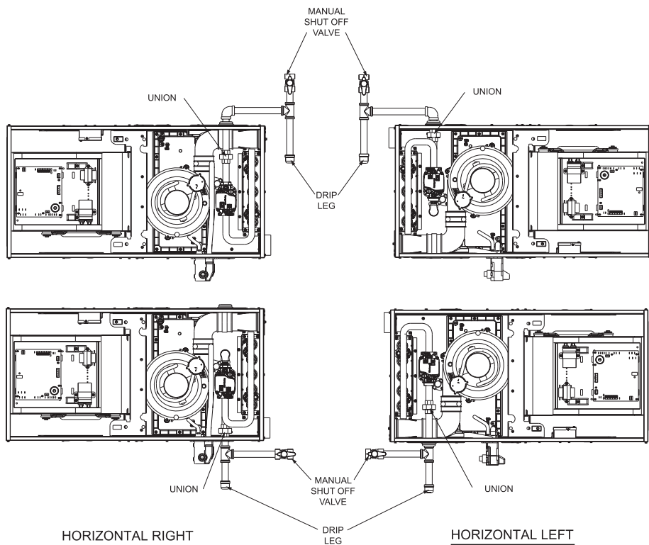
FIGURE 4 BURNER COMPARTMENT - SHOWING LOCATION OF GAS CONTROLS
