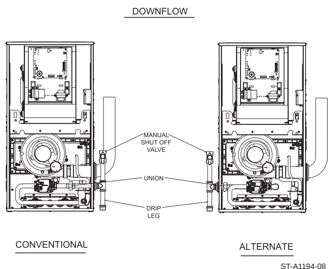
FIGURE 3 BURNER COMPARTMENT - SHOWING LOCATION OF GAS CONTROLS
