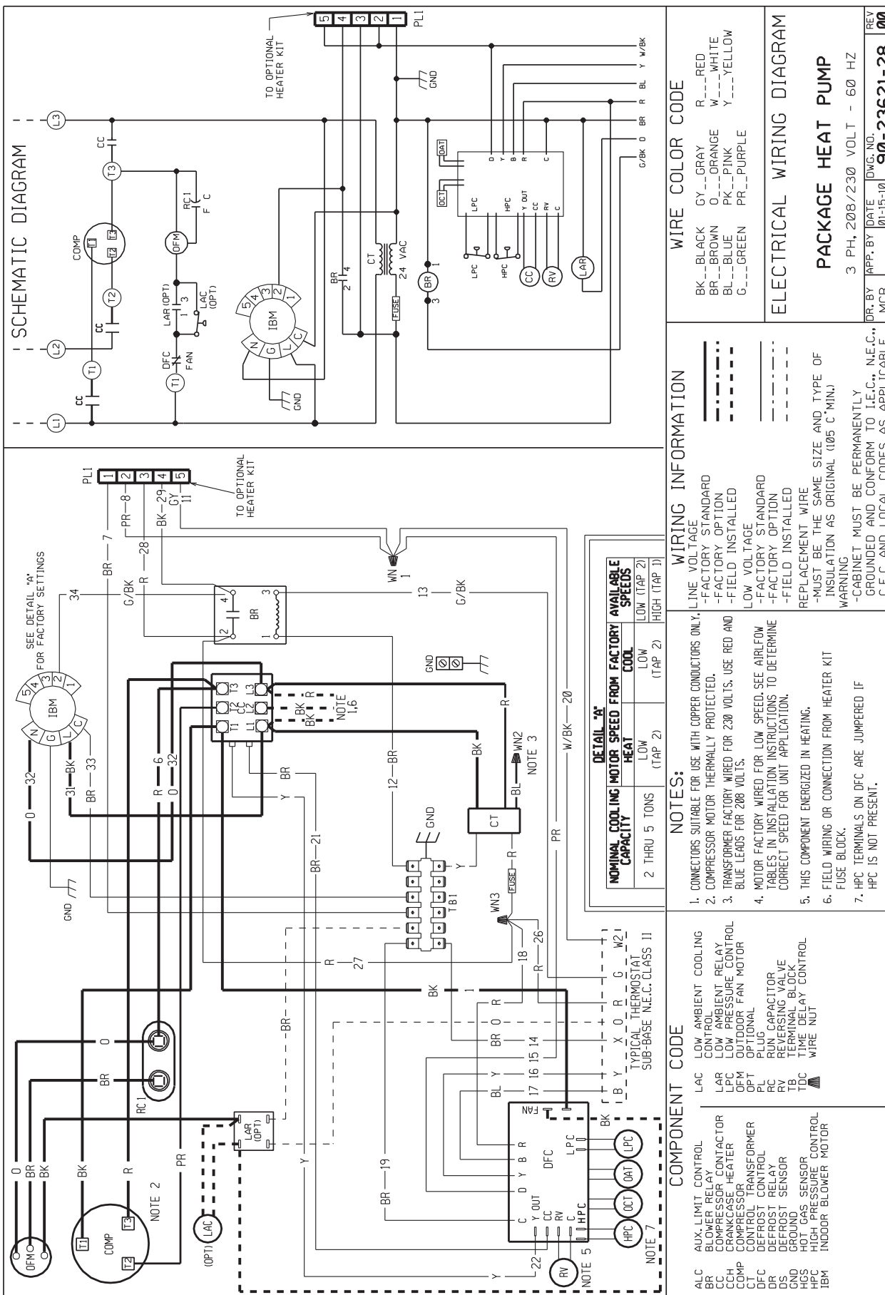
FIGURE 10 WIRING DIAGRAM
