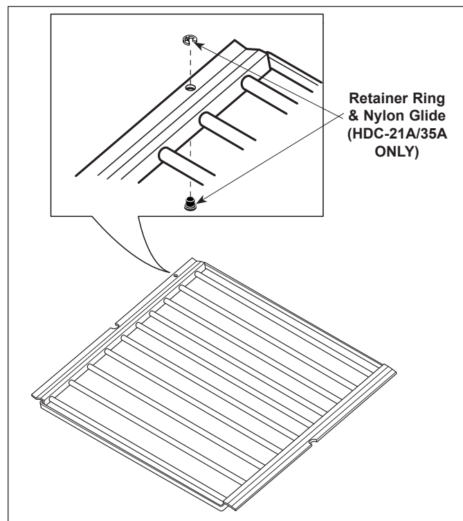
Figure 6. HDC-21A/35A ONLY
