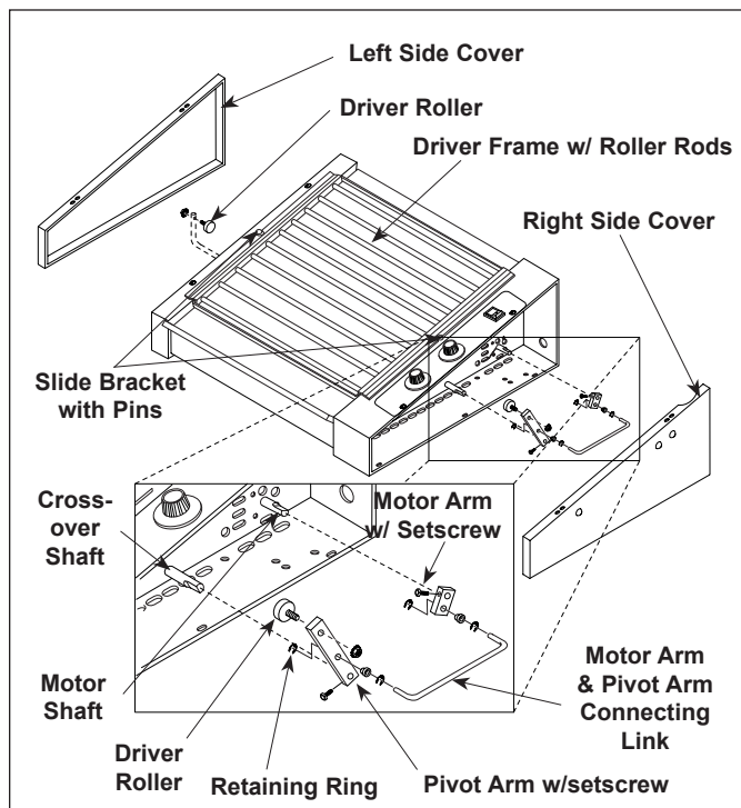
Figure 4. Drive Components
