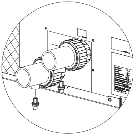
Figure 5. Drain Plugs Locations
