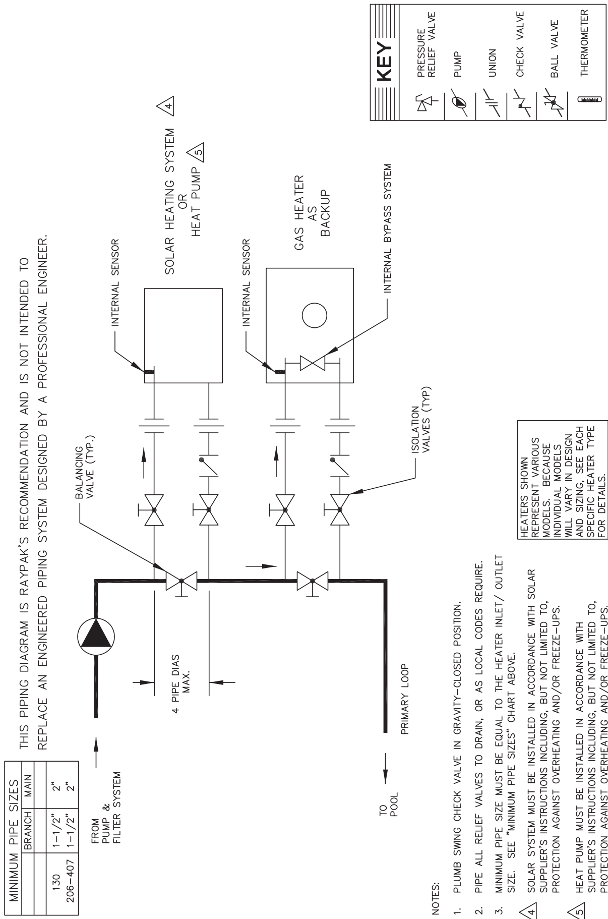
Figure 9. Pool Piping for Heat Pump Pool Heater and Gas Pool Heater
