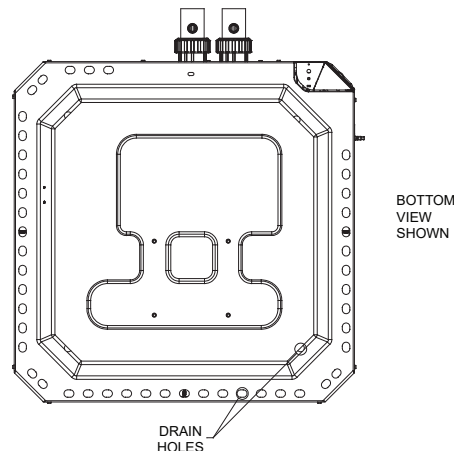
Figure 6. Condensate Drain Hole Locations
