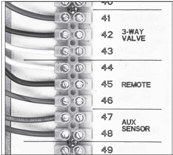
Figure 11. Heater Wiring Block
