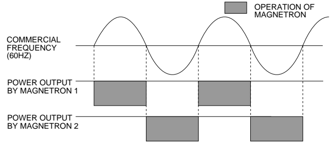
Figure B-1. Operation of Magnetron
