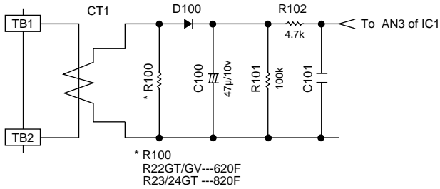
Figure T-1. High Voltage Monitoring Circuit
