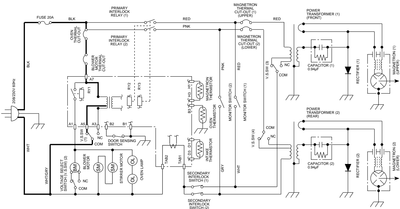
Figure O-1. R-23GT/24GT Oven Schematic-OFF Condition (208 VCondition)
