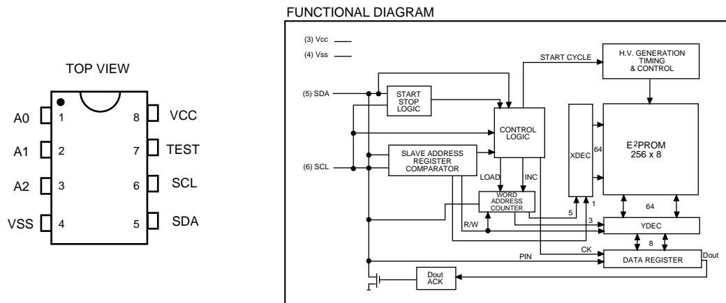
Figure T-4 Relation between Pin Nos. and Signals
