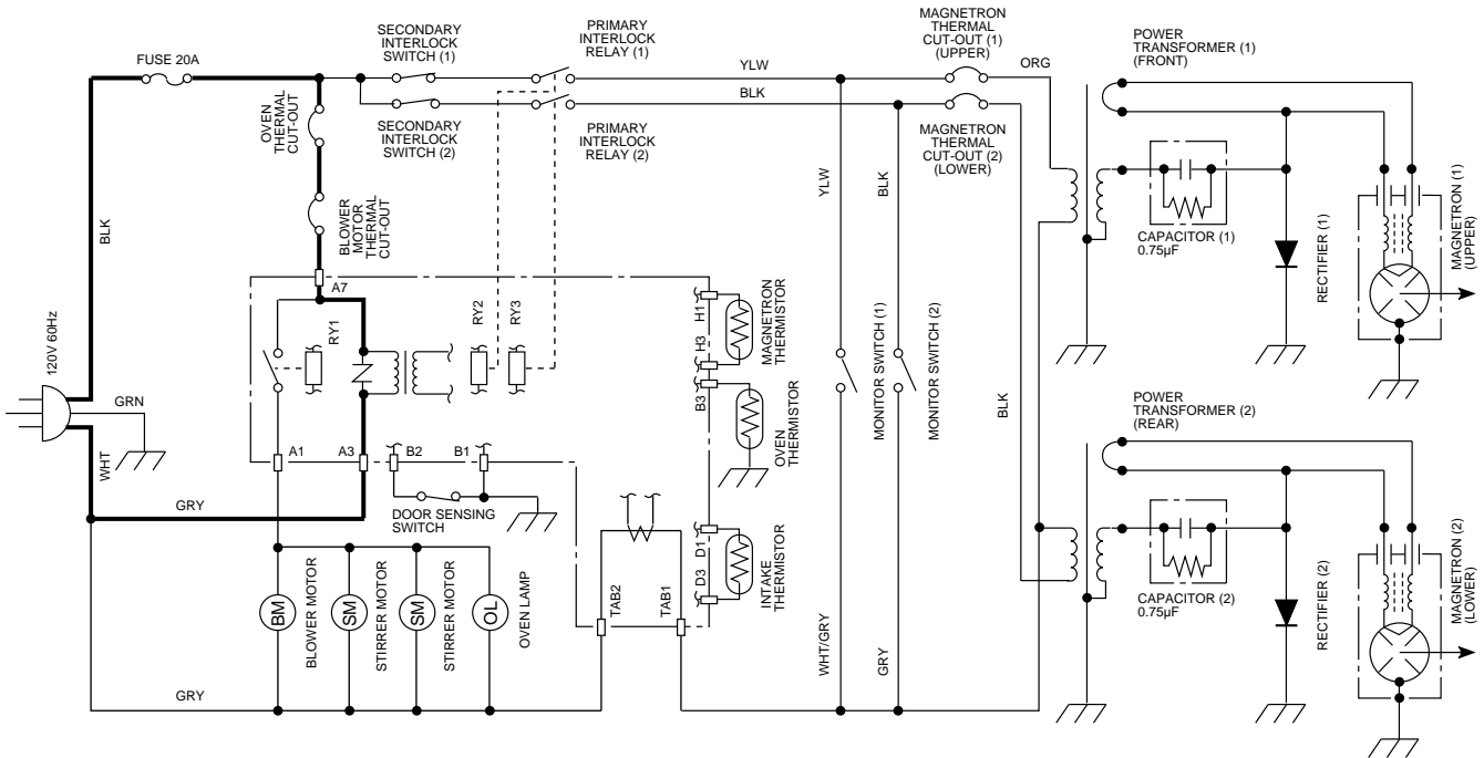
Figure O-1. R-22GV/GT Oven Schematic-OFF Condition
