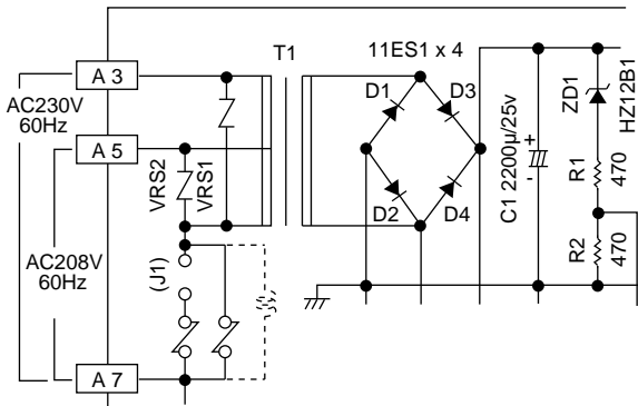
Figure T-2. Supply Voltage Detecting Circuit
