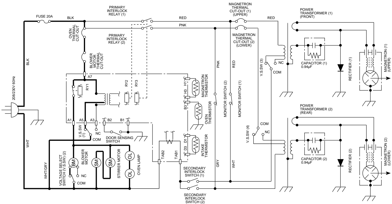
Figure O-2. R-23GT/24GT Oven Schematic-IDLE Condition (208 VCondition)
