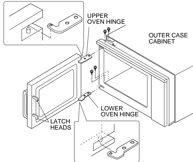
Figure C-3. Door Replacement
