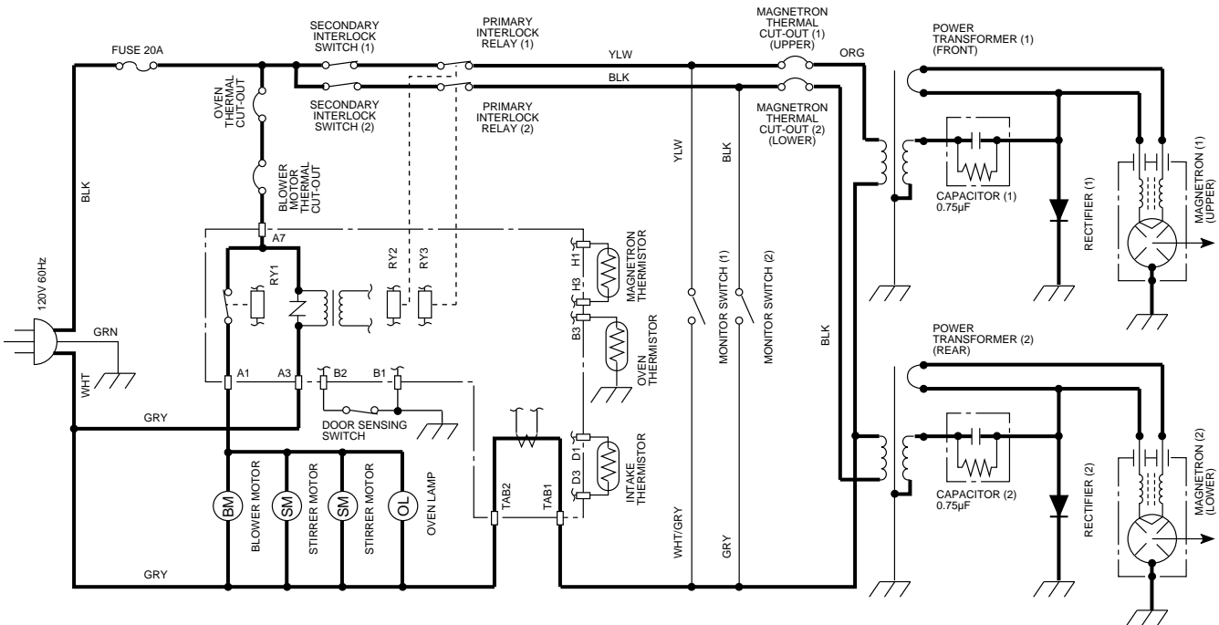
Figure O-3. R-22GV/22GT Oven Schematic-Cooking Condition
