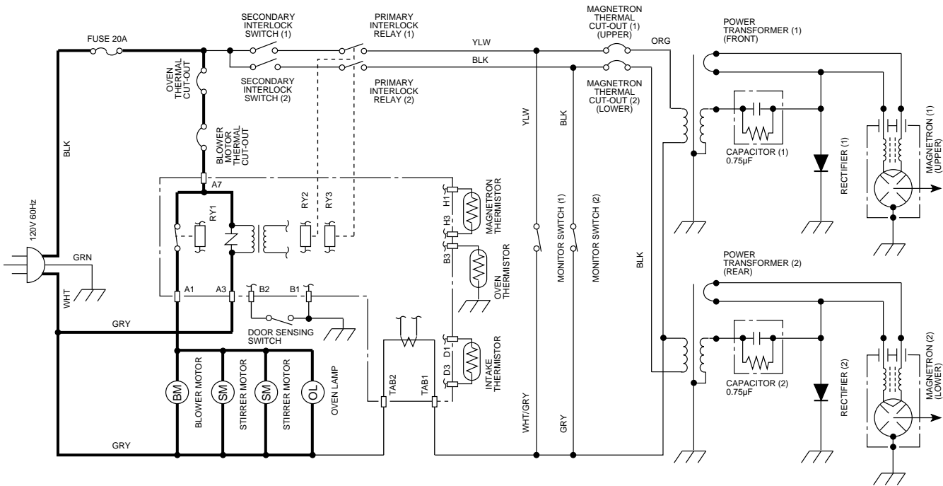
Figure O-2. R-22GV/22GT Oven Schematic-IDLE Condition
