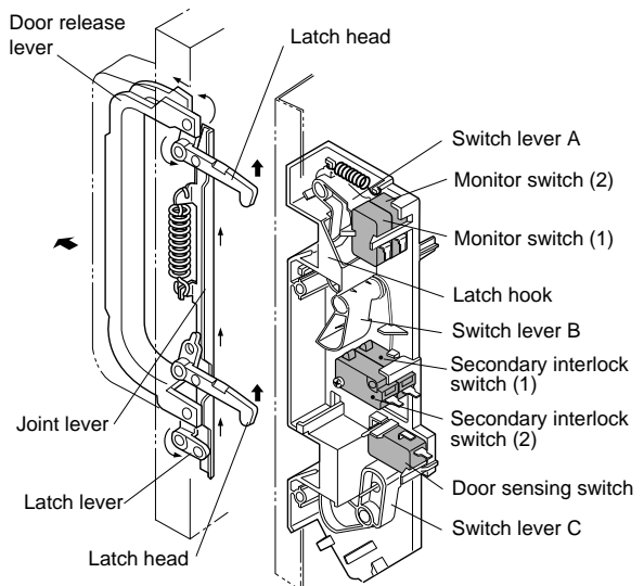
Figure C-2. Latch Switch Adjustments
