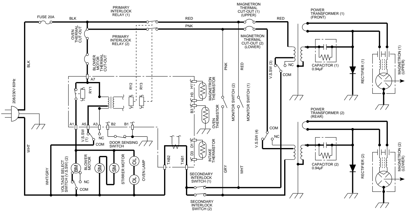
Figure O-3. R-23GT/24GT Oven Schematic-Cooking Condition (208 V Condition)
