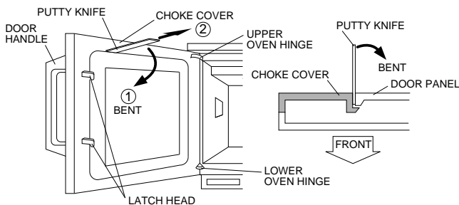
Figure C-4. Choke cover
