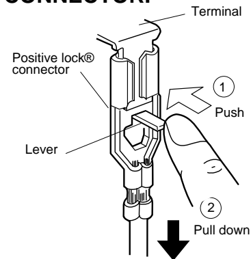
Figure C-1. How to release the positive lock connector.
