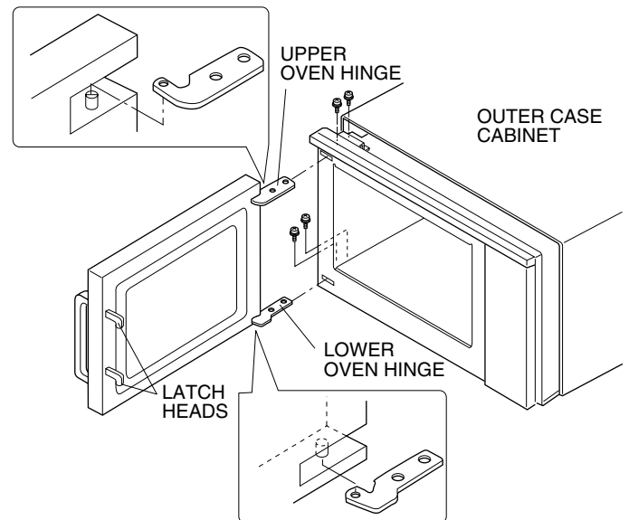
Figure C-4. Door Replacement
