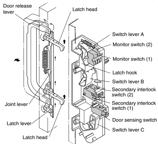
Figure C-3. Latch Switch Adjustments
