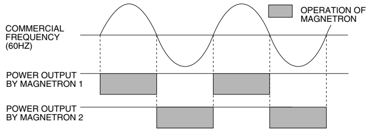
Figure B-1. Operation of Magnetron
