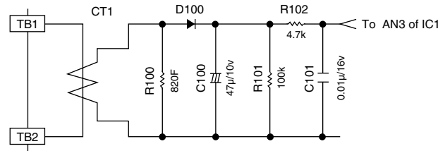
Figure T-1. High Voltage Monitoring Circuit
