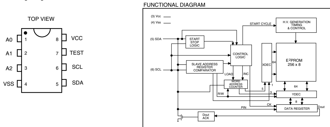
Figure T-3 Relation between Pin Nos, and Signals
