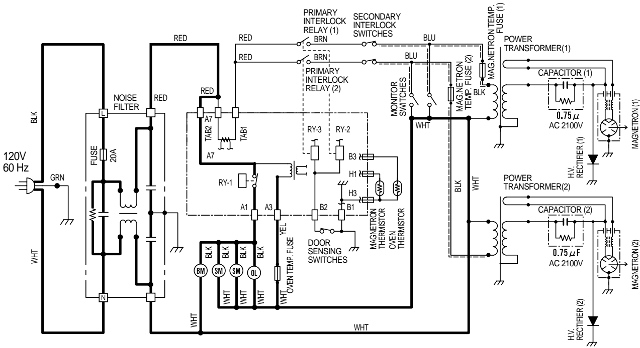
Figure O-2. Oven Schematic-IDLE Condition (208 V Condition)
