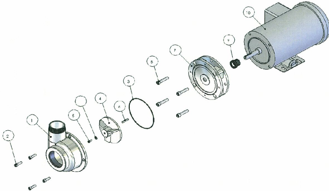
FIGURE 2. KW DIRECT DRIVE PUMP EXPLODED VIEW
