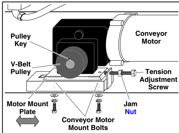
Figure 9: Conveyor Motor V-Belt Tension Adjustment
