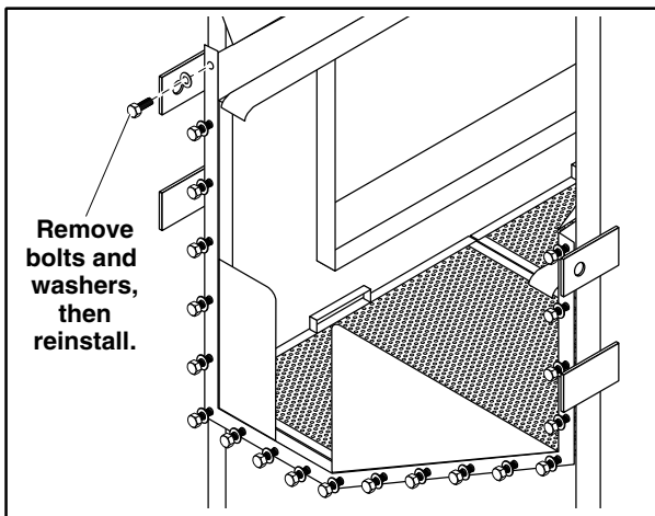
Figure 2: Load End Tank Mount
