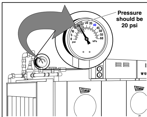
Figure 19: Final Rinse Pressure
