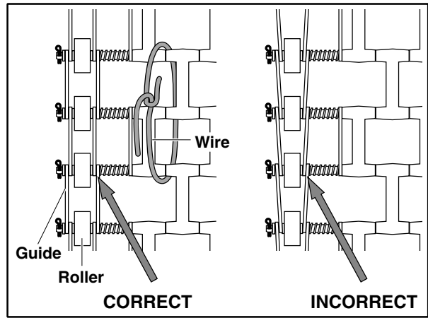
Figure 13: Conveyor Peg Belt Assembly
