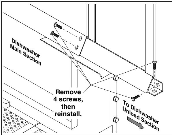
Figure 8: Unload Belt Roller Guard Extension
