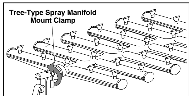
Figure 28: Tree-Type Spray Manifold Mounting Clamp Handle
