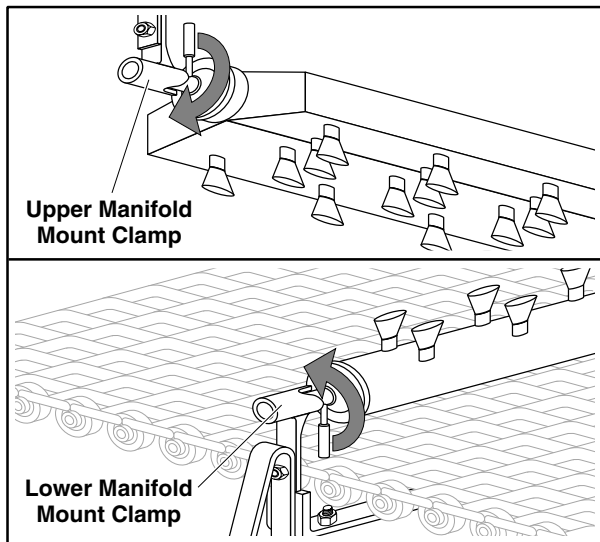
Figure 26: Scrapper Spray Manifold Mount Clamp
