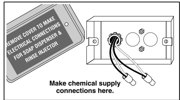
Figure 21: Chemical Supply Connection
