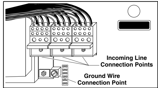
Figure 20: Main Electrical Connection
