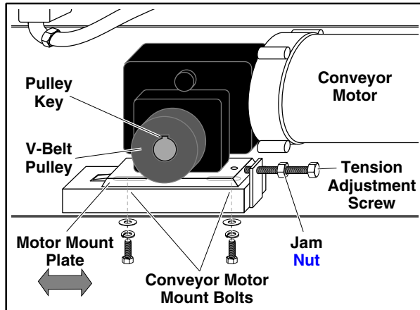
Figure 22: Conveyor Motor V-Belt Tension Adjustment
