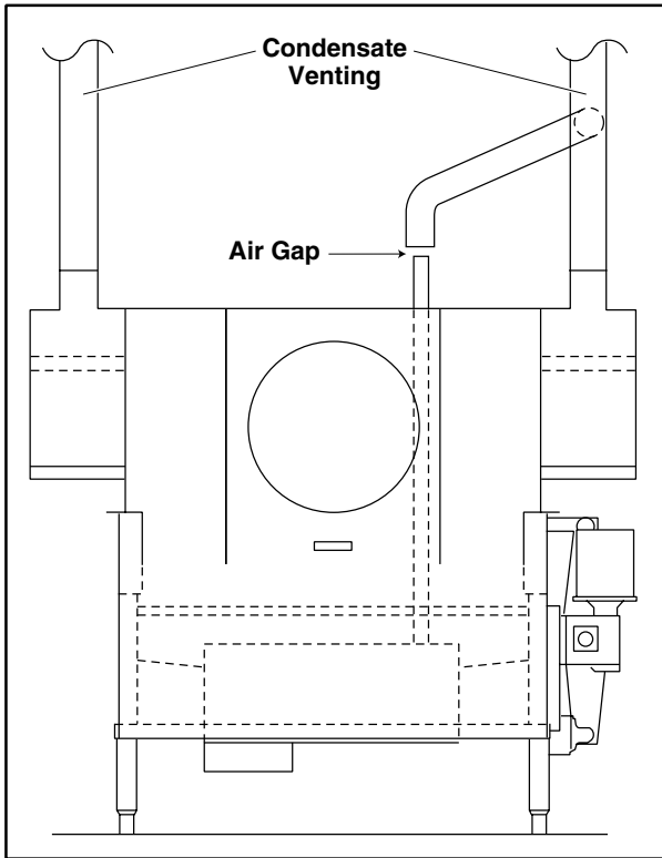
Figure 17: Recommended Gas Venting
