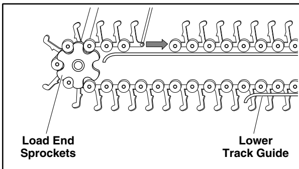
Figure 12: Lower Track Guides
