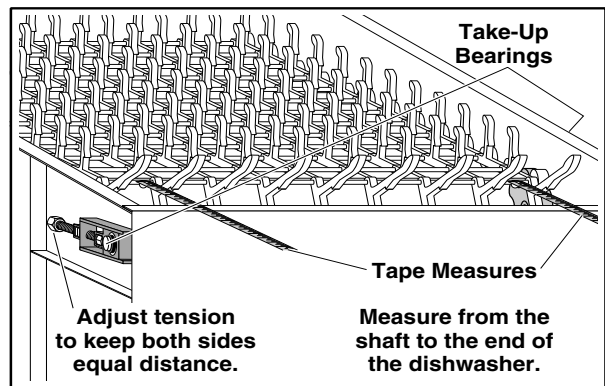
Figure 14: Take-up Bearing Adjustment
