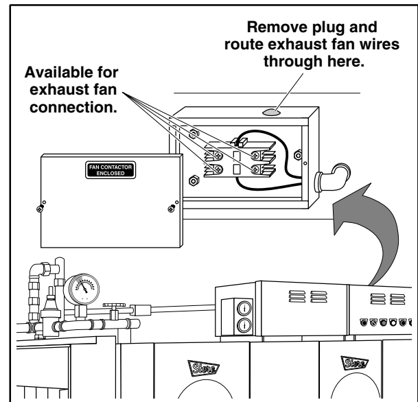
Figure 18: Exhaust Fan Electrical Connection
