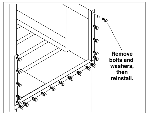
Figure 6: Unload End Tank Mount
