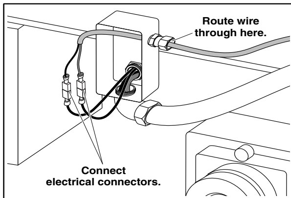
Figure 15: Conveyor Stop Bar Switch Electrical Connection
