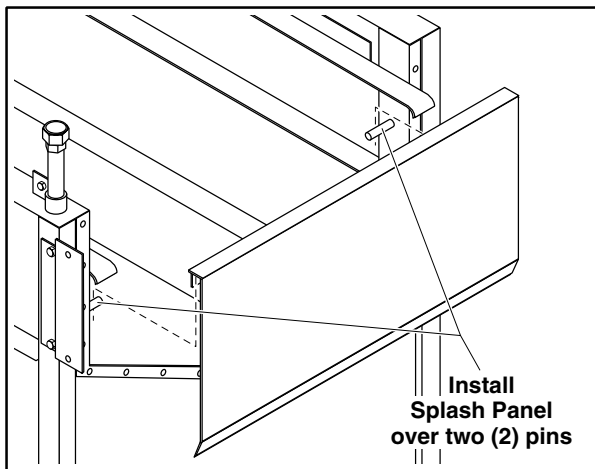
Figure 5: Splash Back Panel Installation
