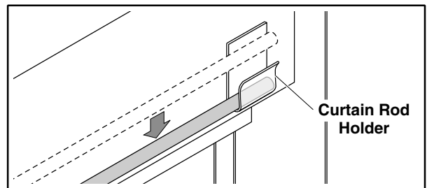
Figure 16: Curtain Rod Holder
