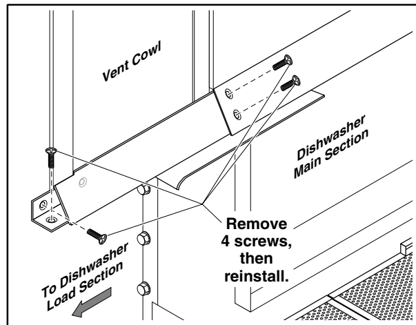
Figure 4: Load Belt Roller Guard Extension
