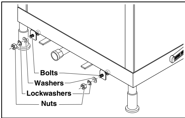
Figure 7: Unload End Frame Mount
