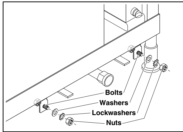
Figure 3: Load End Frame Mount
