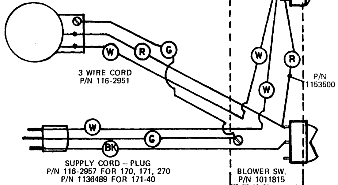
CONNECTION DIAGRAM
