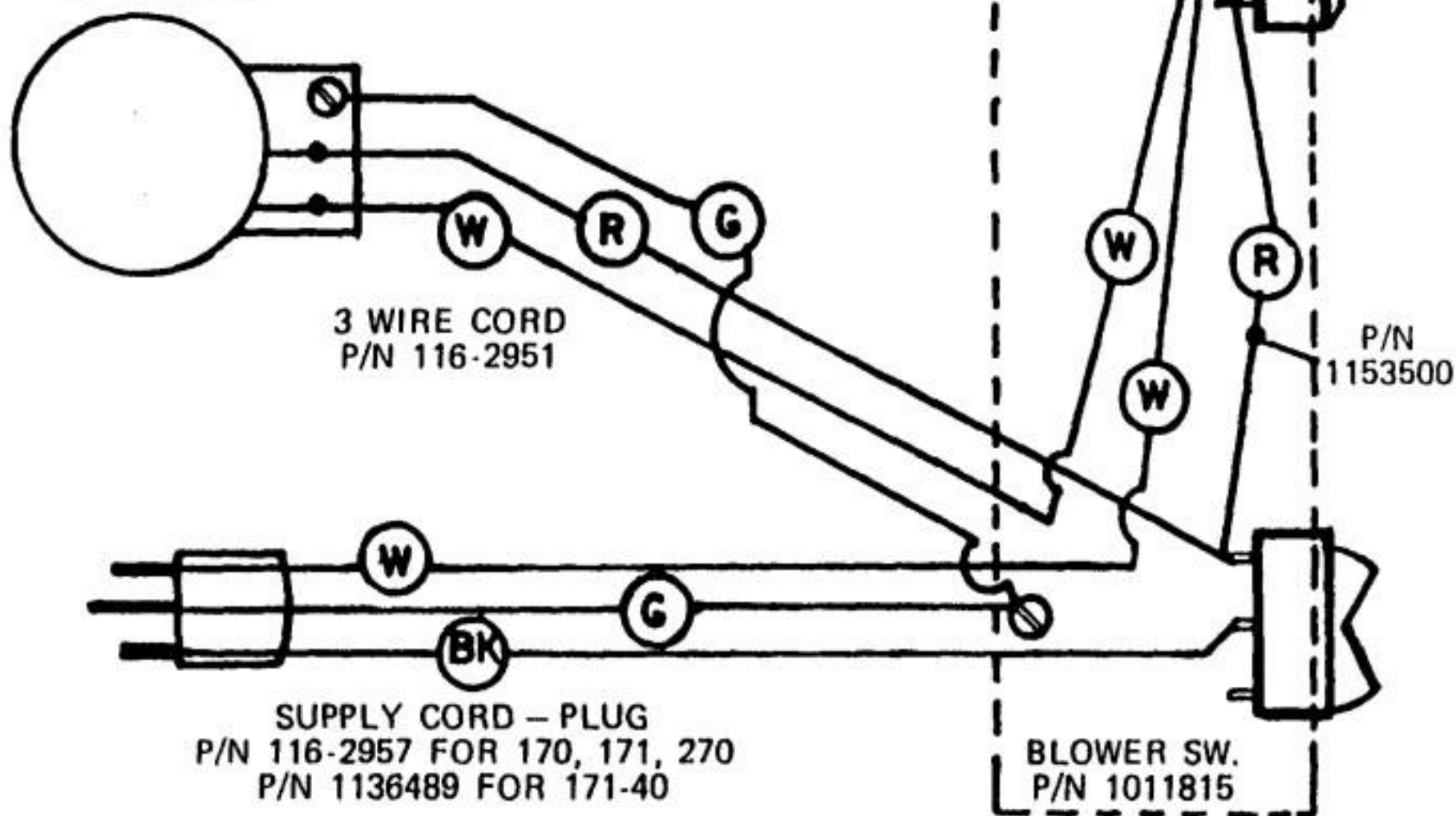
CONNECTION DIAGRAM
