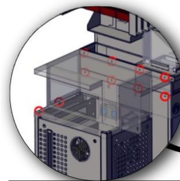
Eight 7/16" Hex Bolts Two 7/16" Cap Nuts
