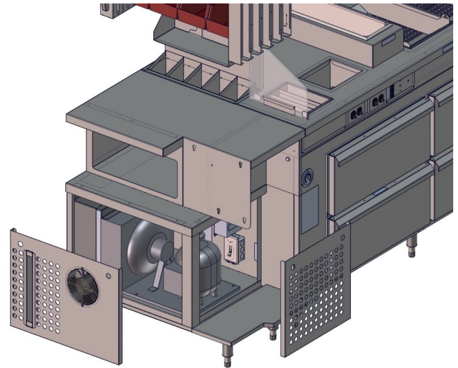
Removable Panels
