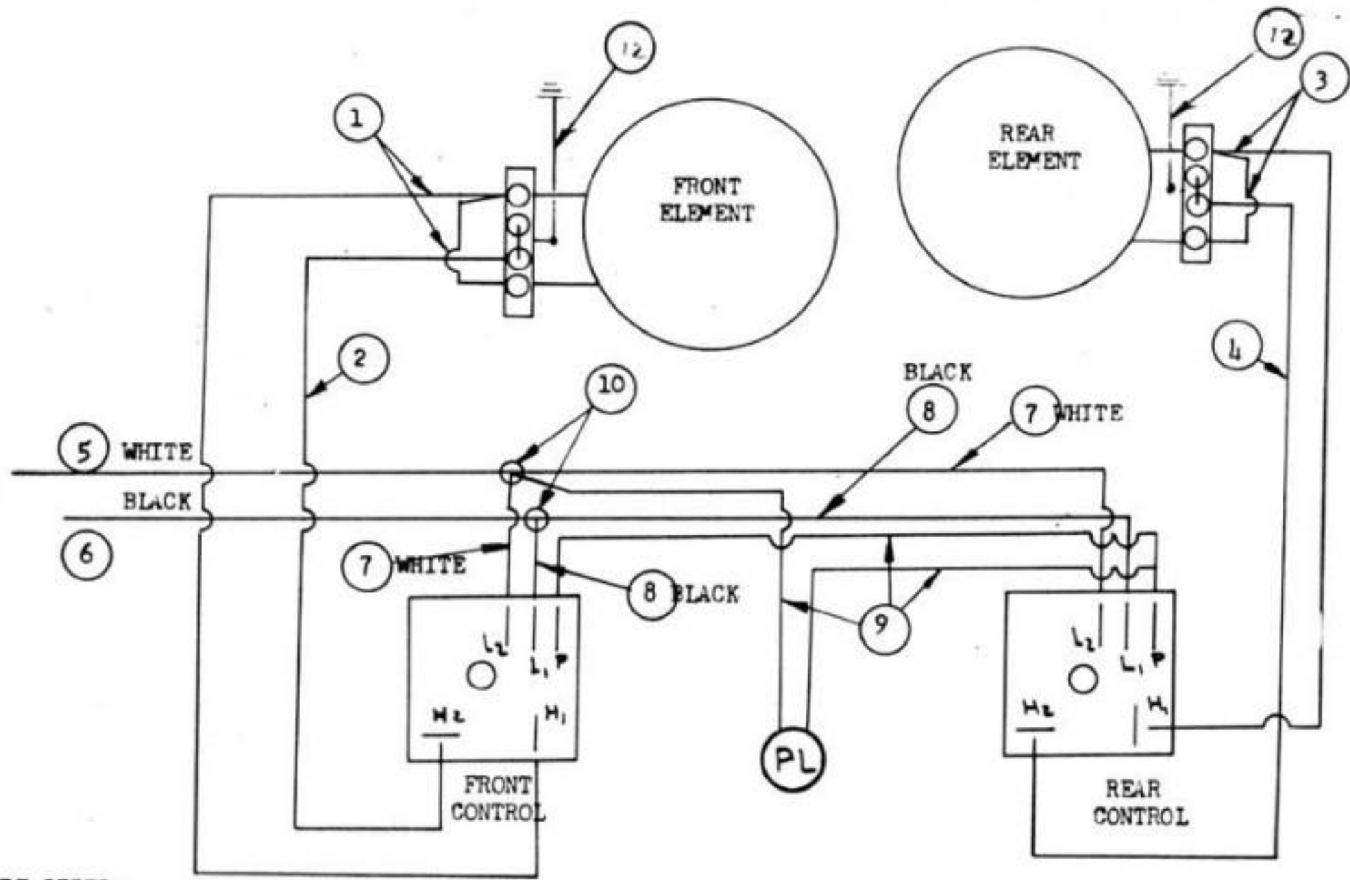
CONTROLS VIEW FROM FRONT OF UNIT
