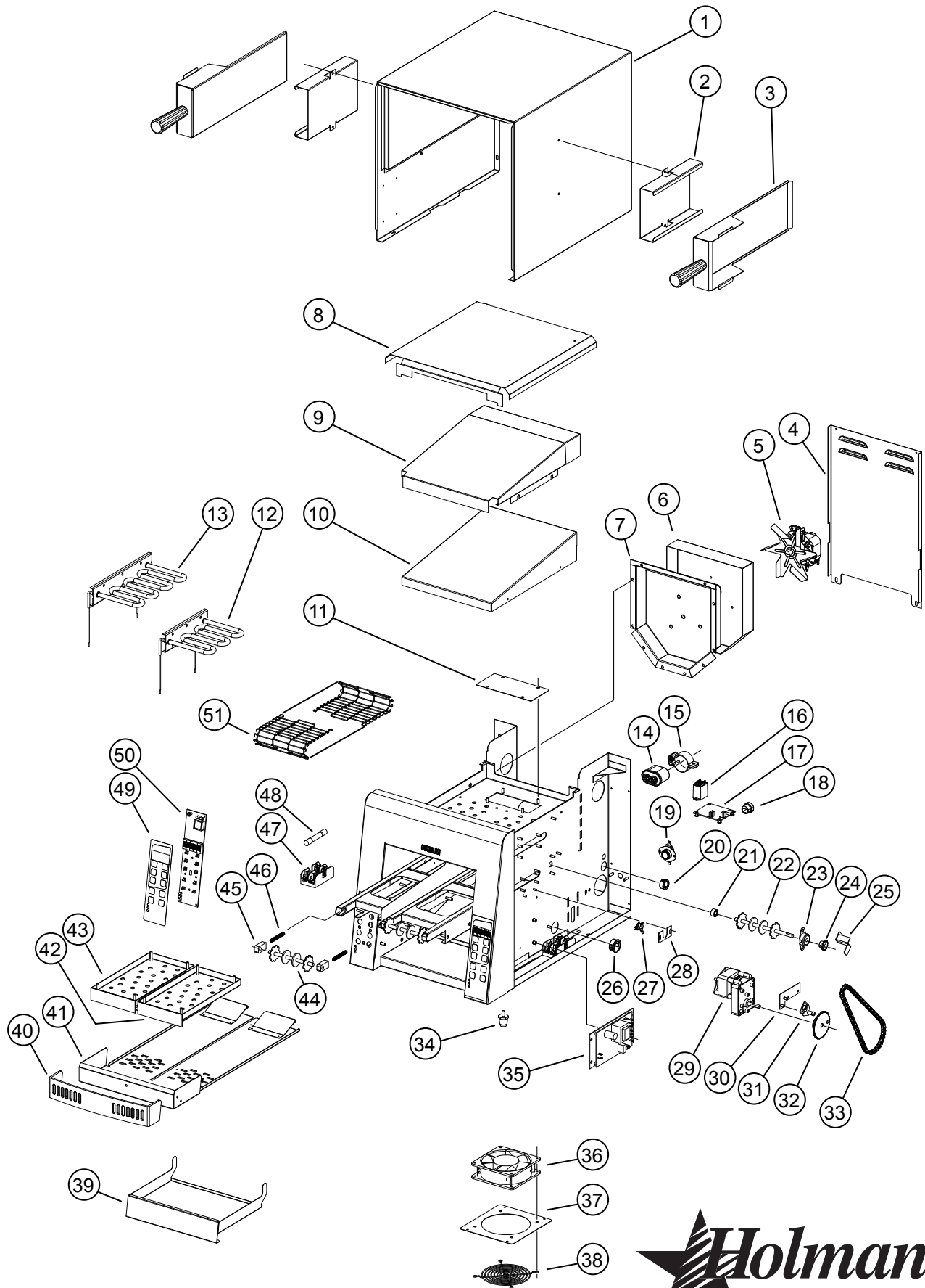
MODEL: IRCS2-SB: Split Electronic Conveyor Toaster
