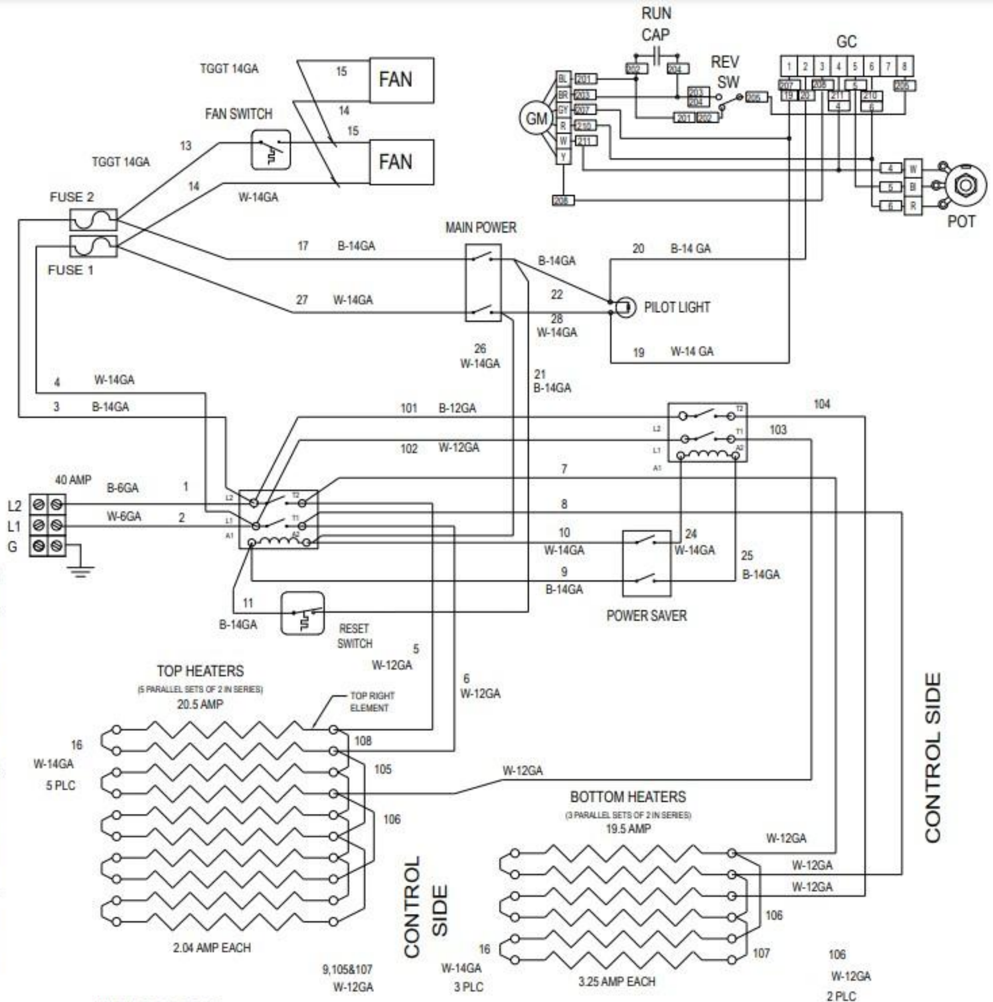
WIRING DIAGRAM QT14-REV "D"
