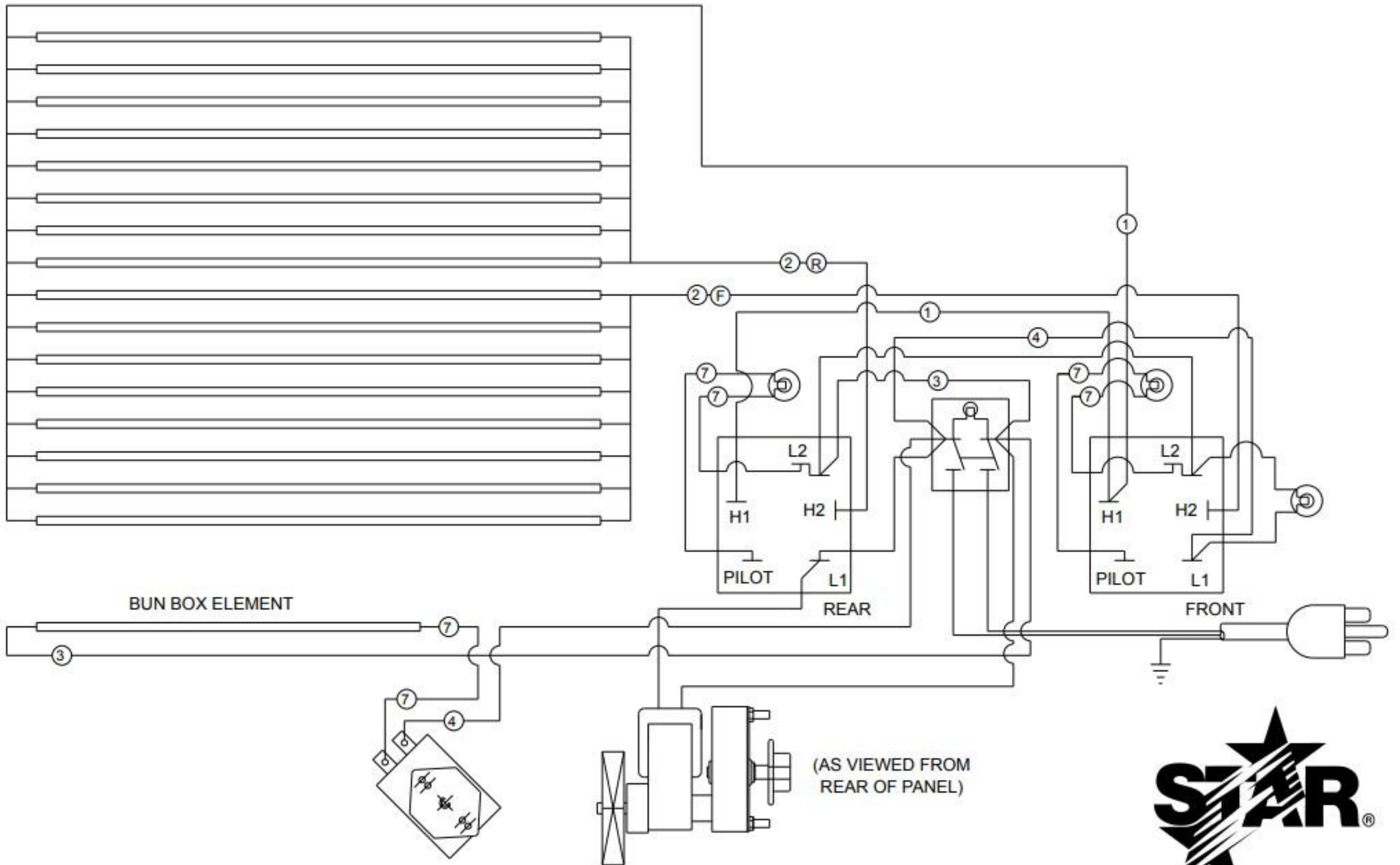
50SCHDM=120V WIRE DIAGRAM
