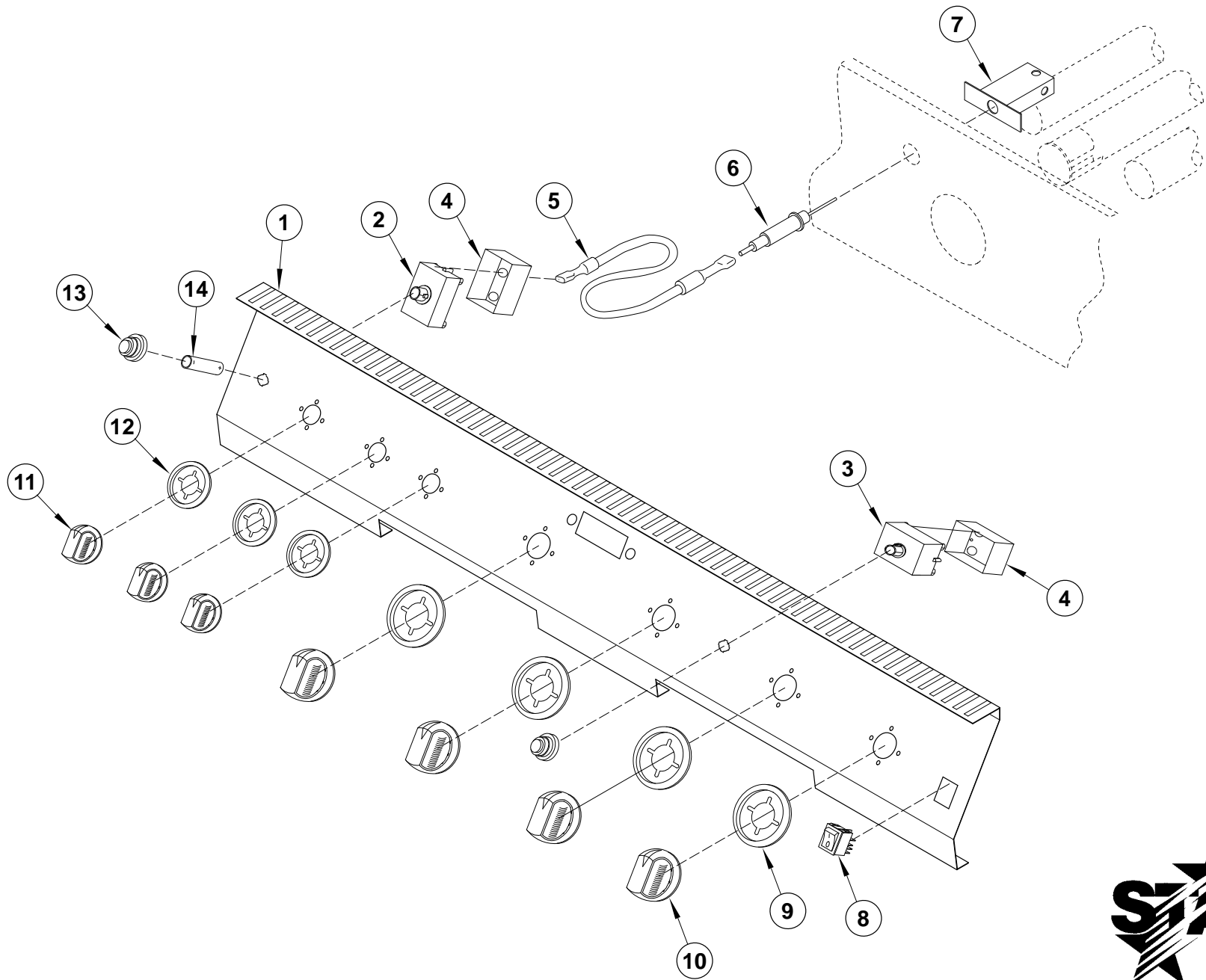
TYPICAL FACEPLATE ASSEMBLY - MODEL SSG48 SHOWN REFER TO THE PARTS LIST SPECIFIC TO YOUR MODEL FOR MORE DETAIL INFORMATION.
