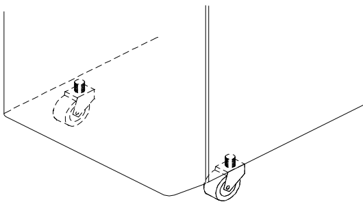
Figure 6. Caster Adjustment
