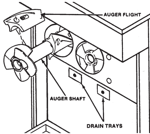
Figure 24. Auger Shafts
