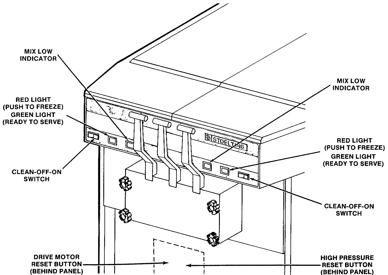
Figure 9. Controls
