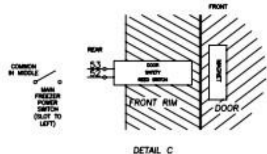
DETAIL C
