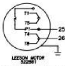
DETAIL A (CF101 230 V APPLICATION)
