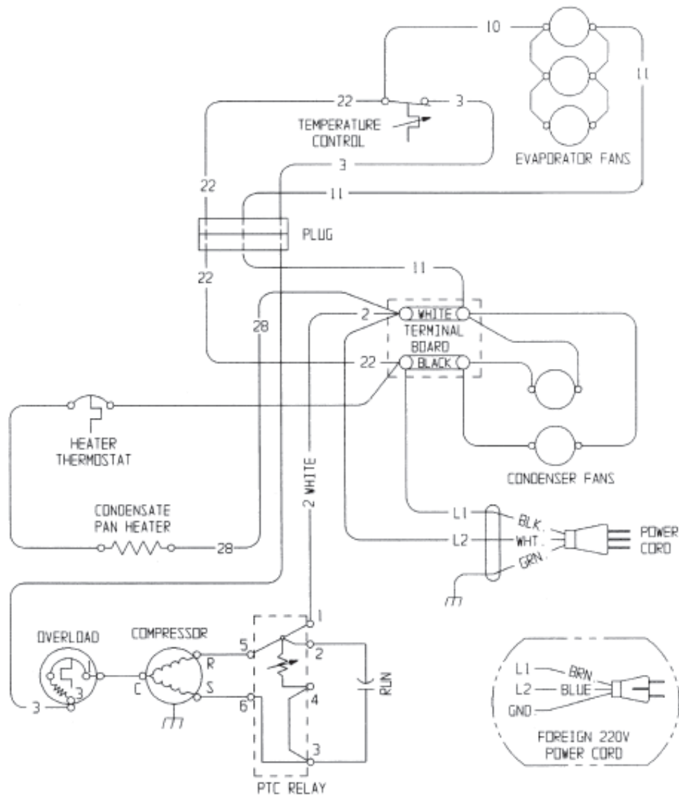
WIRING DIAGRAM Model: SKP6016 115V, 60Hz, 1 PH OR 220V, 50/60 Hz, 1 PH
