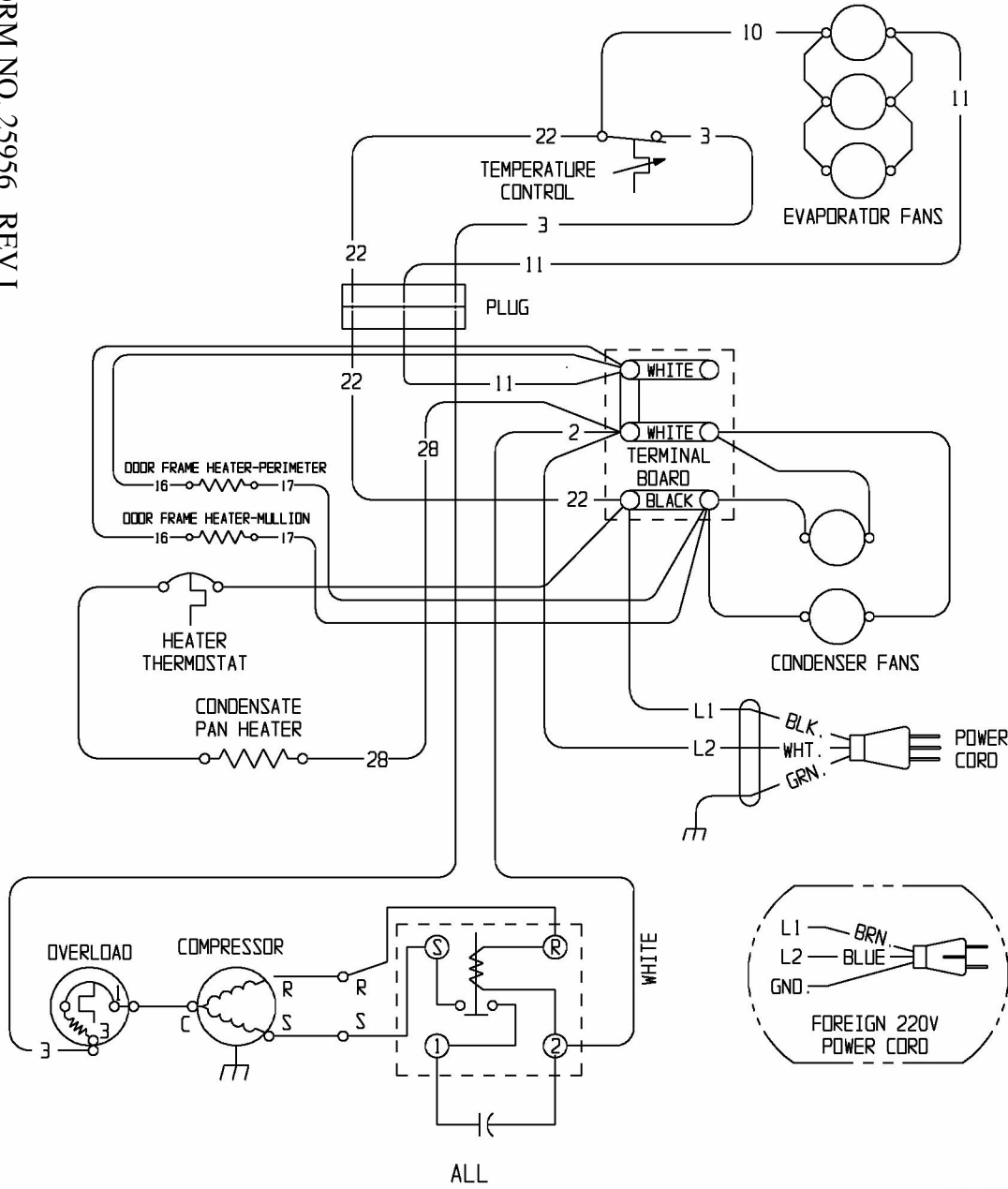
WIRING DIAGRAM
