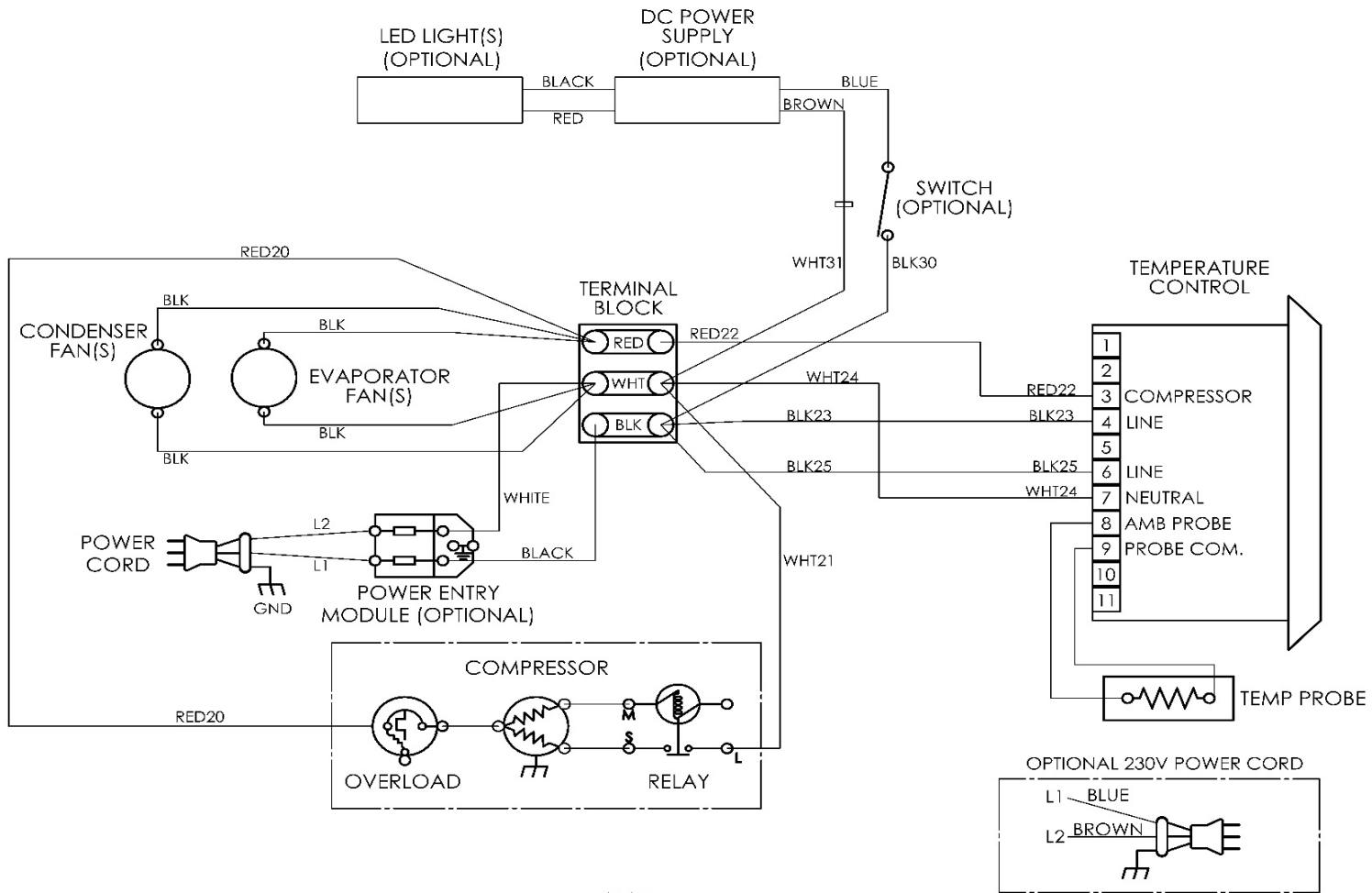
46451 WIRING DIAGRAM REV A
