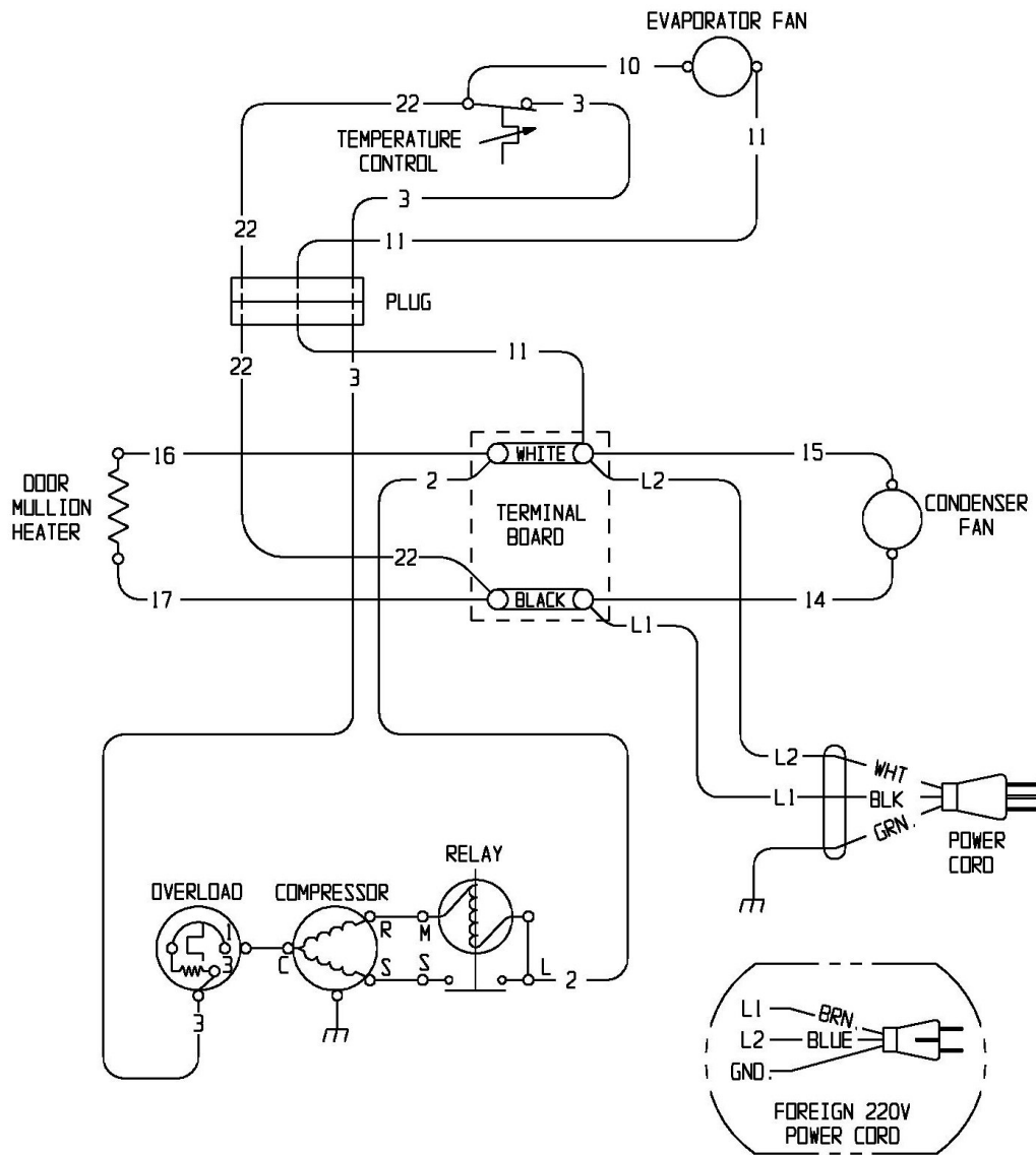
WIRING DIAGRAM MODEL SKSR
