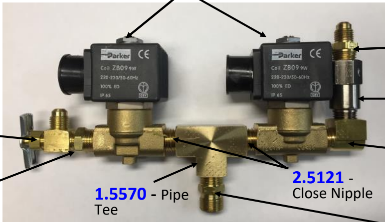
3.6110 S Series Water Control Assembly Complete -
