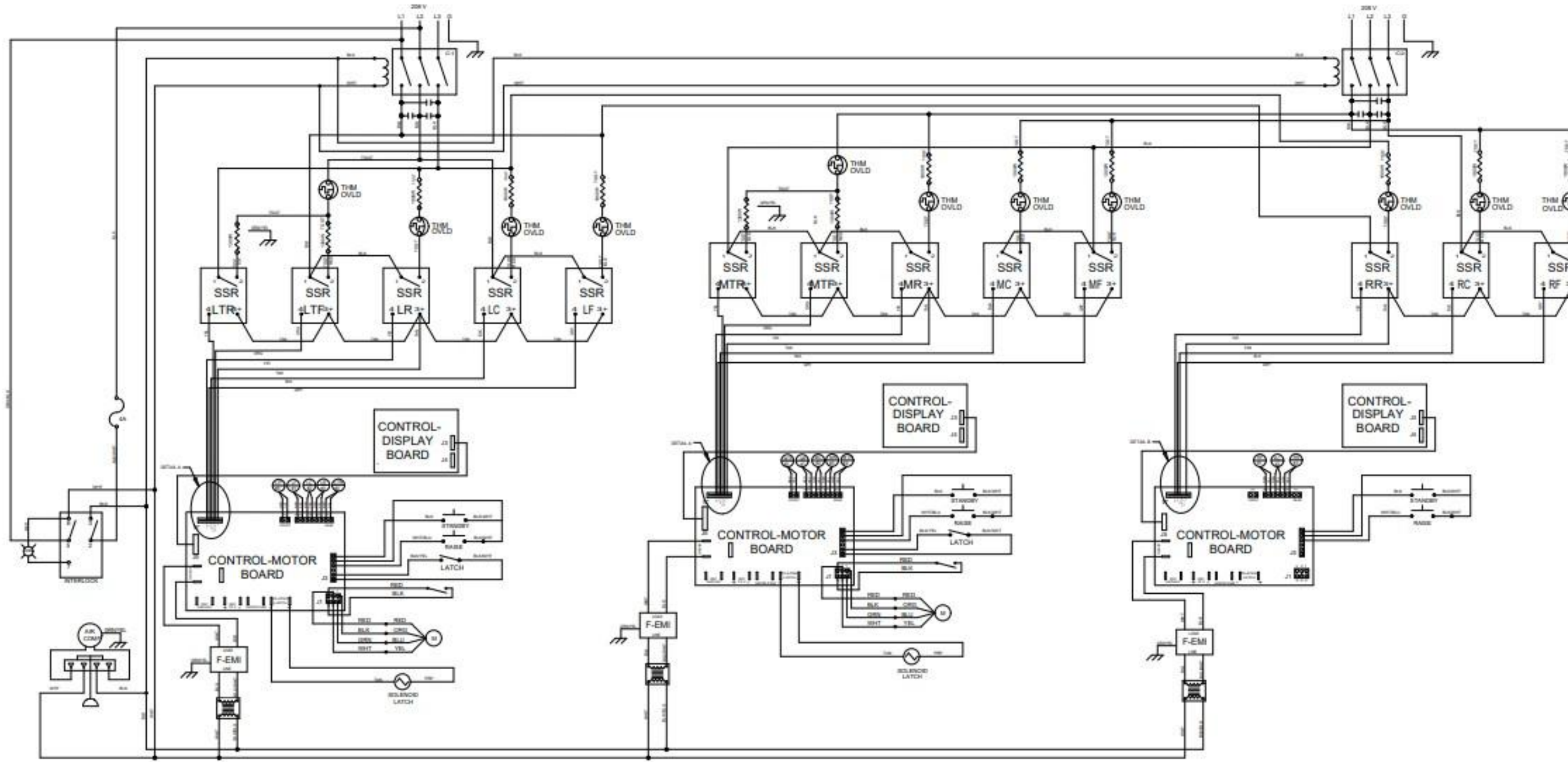
DETAIL B
