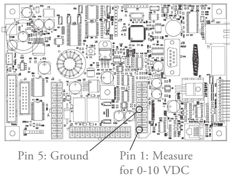
Figure 20: SAGE Control Board, Blower Test Points
