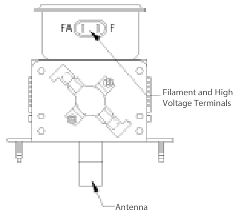
Figure 31: Magnetron Detail
