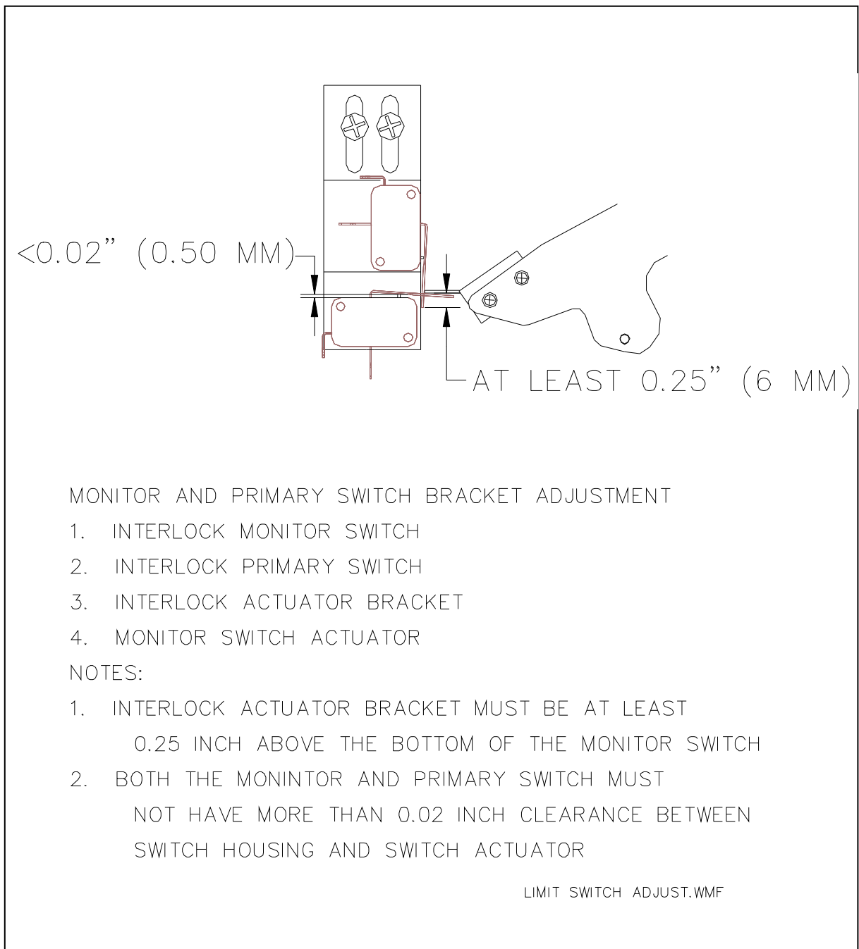
Figure 7-58: Interlock Switch Adjustment
