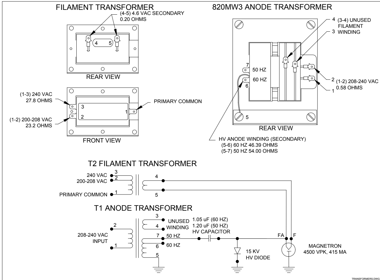
FIGURE 9-4 Transformer Testing
