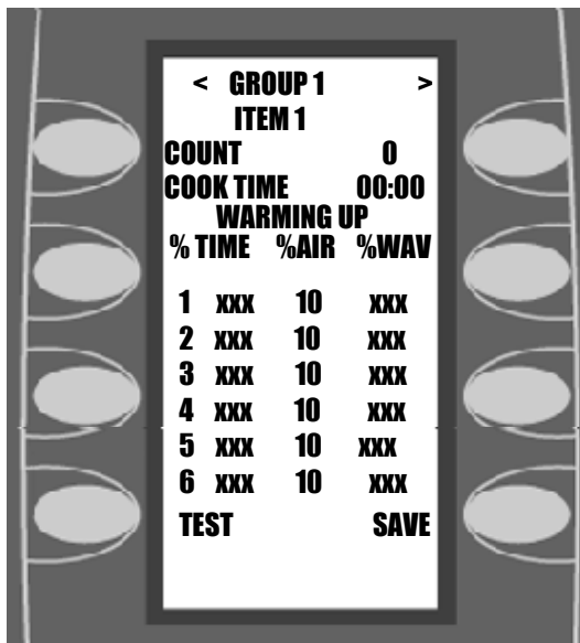
Figure 3-3: Edit Groups
