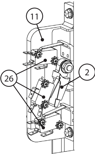
Figure A-7: Door Switch Assembly
