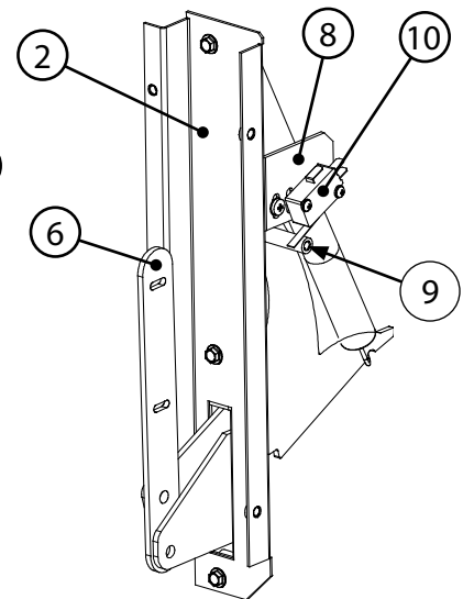
Figure 42: Right Hinge Detail
