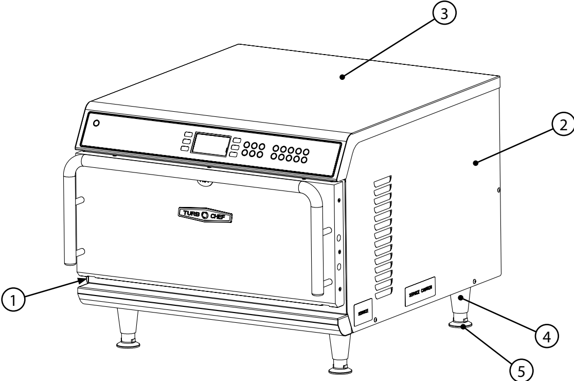
Figure 44: Miscellaneous Components
