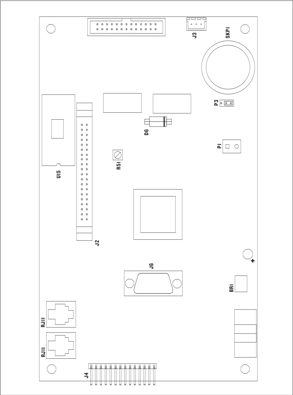
FIGURE 62: I/O Control Board and Test Point Locations
