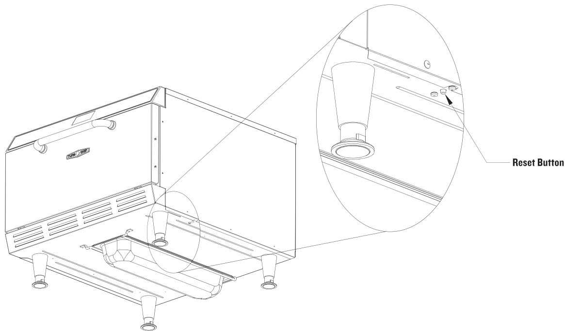
FIGURE 25: Location of Hi-Limit Thermostat Reset Button
