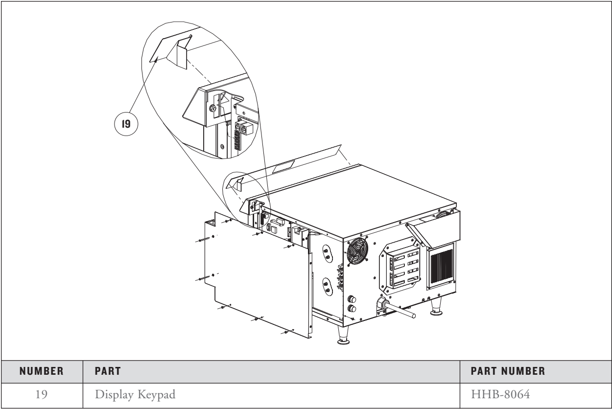
FIGURE 42: Replacing the Display Keypad
