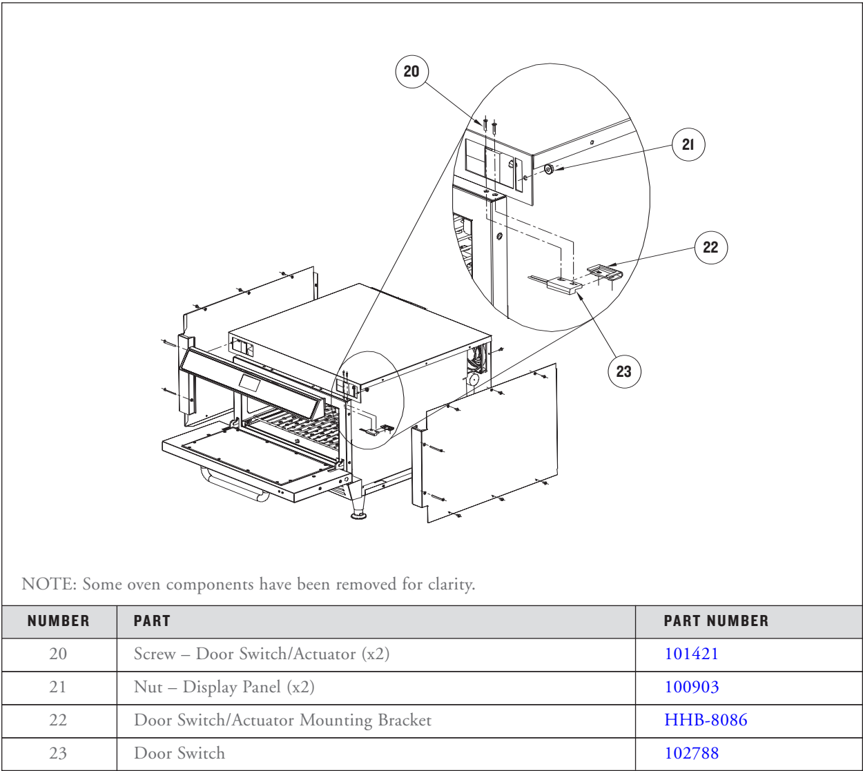
FIGURE 43: Replacing the Door Switch
