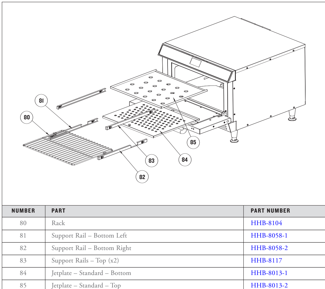
FIGURE 57: Removing Jetplates
