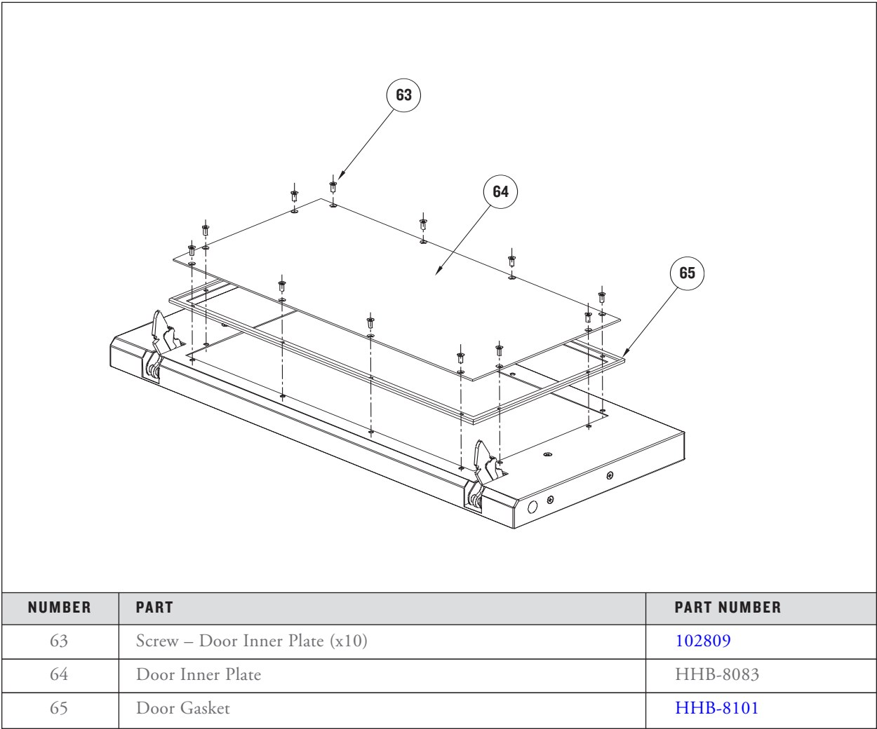
FIGURE 52: Removing the Door Gasket
