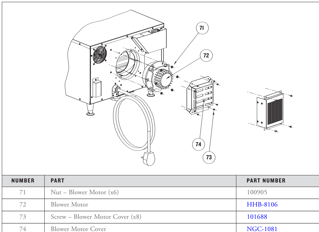
FIGURE 55: Removing the Blower Motor
