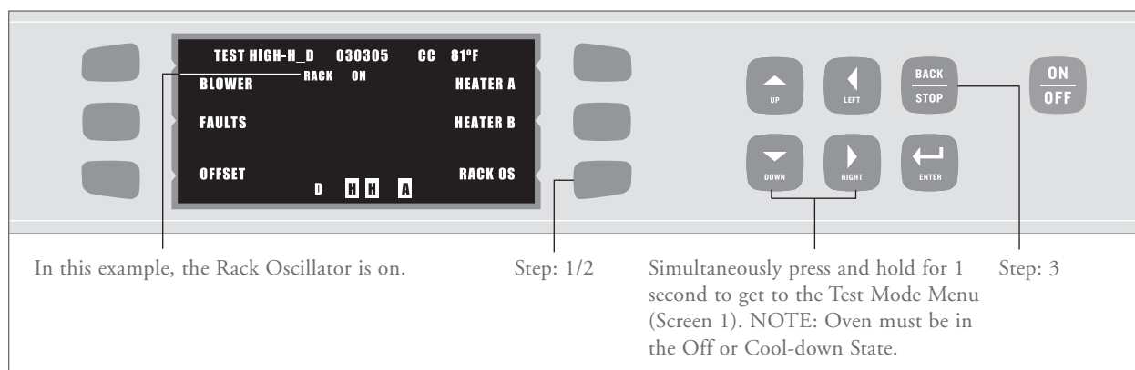
FIGURE 32: Testing the Rack Oscillator
