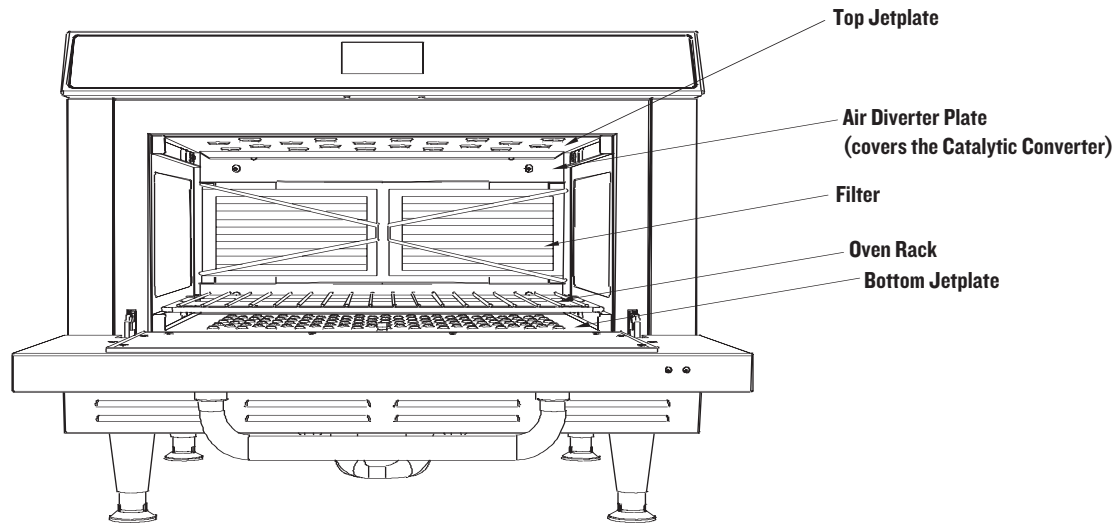
FIGURE 60: The Cook Chamber
