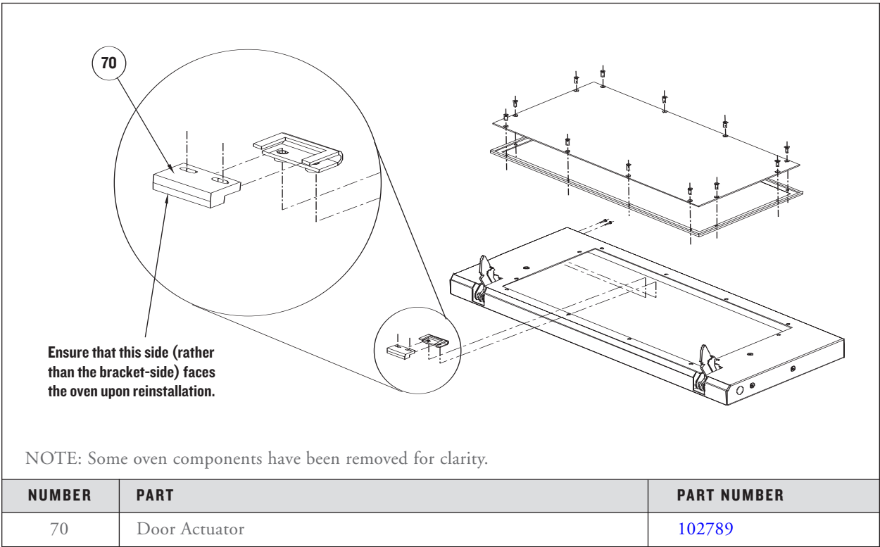
FIGURE 54: Door Actuator and Mounting Bracket
