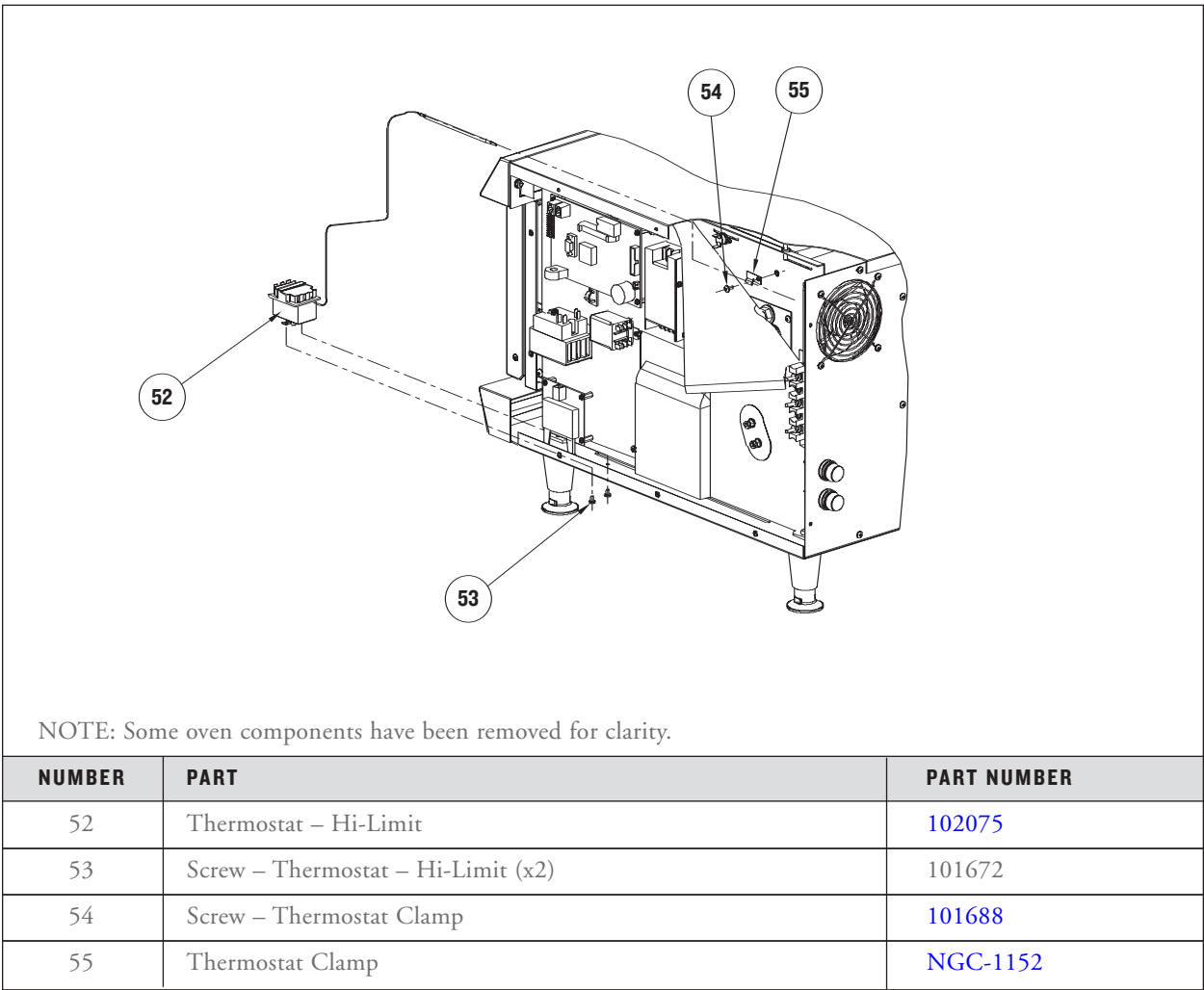
FIGURE 49: Removing the Hi-Limit Thermostat
