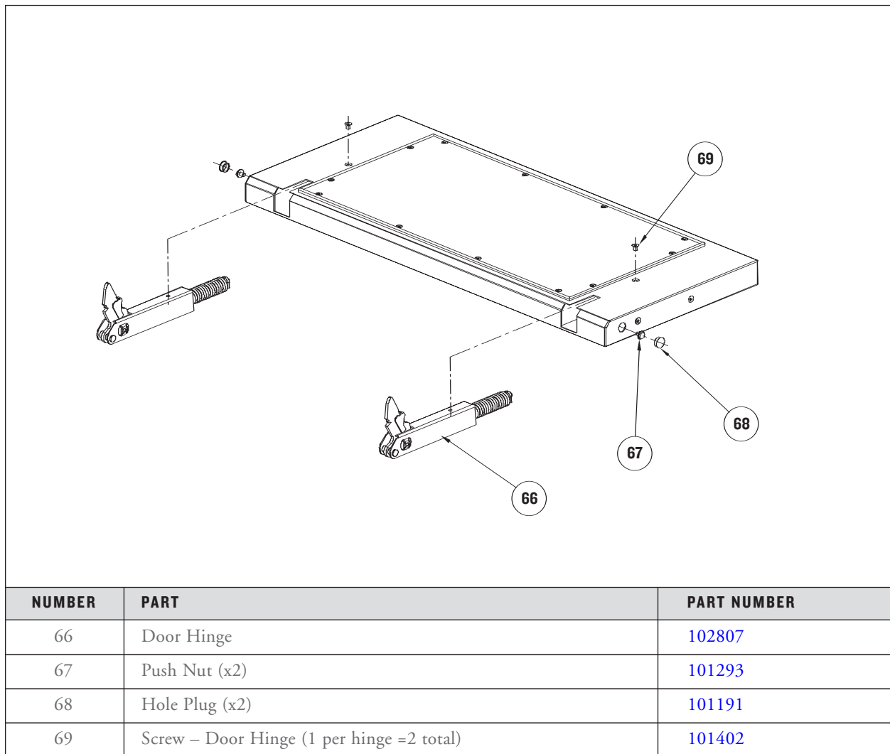
FIGURE 53: Replacing a Hinge
