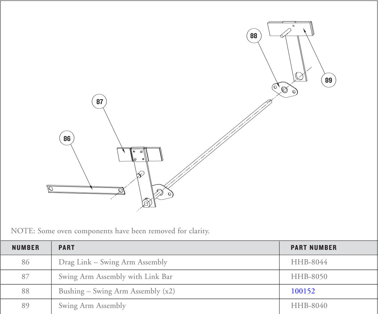
FIGURE 58: Swing Arm Assembly
