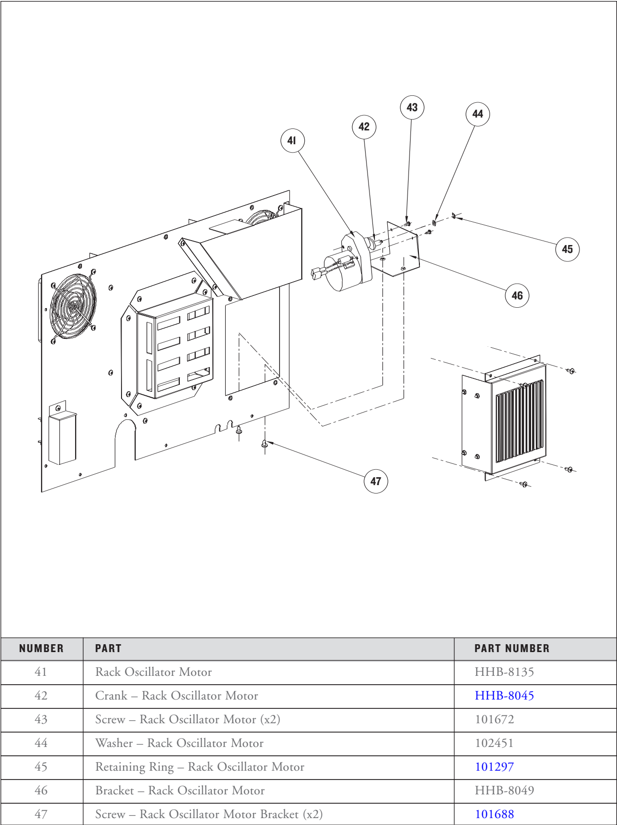
FIGURE 46: Removing the Rack Oscillator Motor
