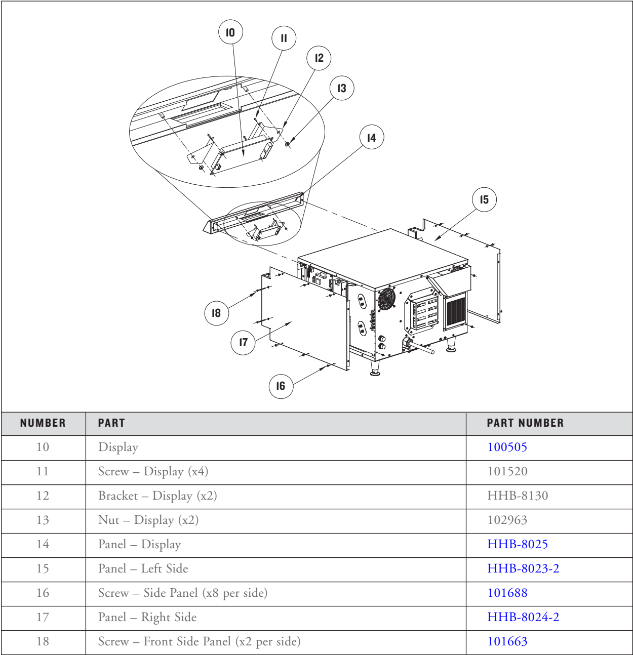
FIGURE 4I: Replacing the Display
