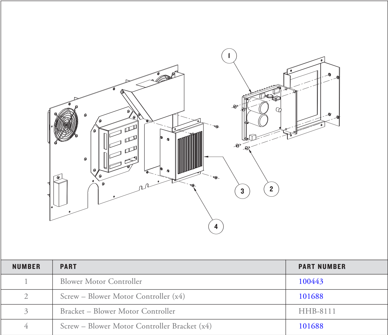
FIGURE 39: Removing Blower Motor Controller
