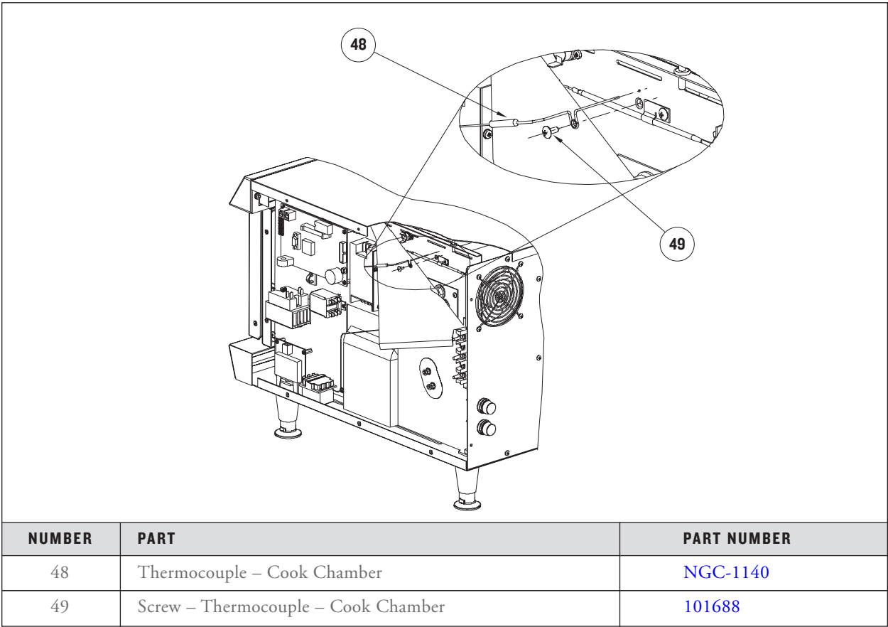
FIGURE 47: Removing the Cook Chamber (CC) Thermocouple
