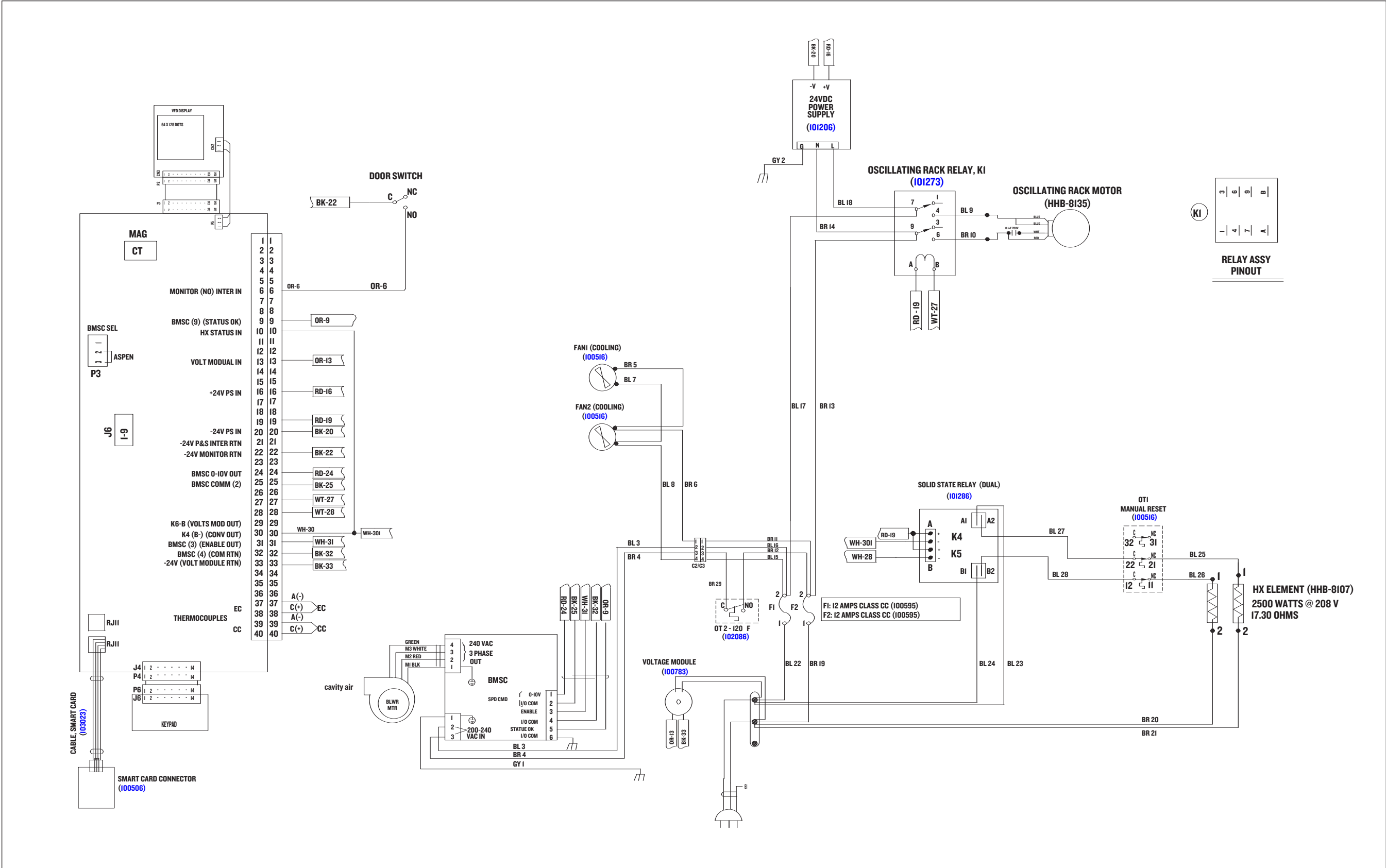
FIGURE 61: High h Batch Schematic
