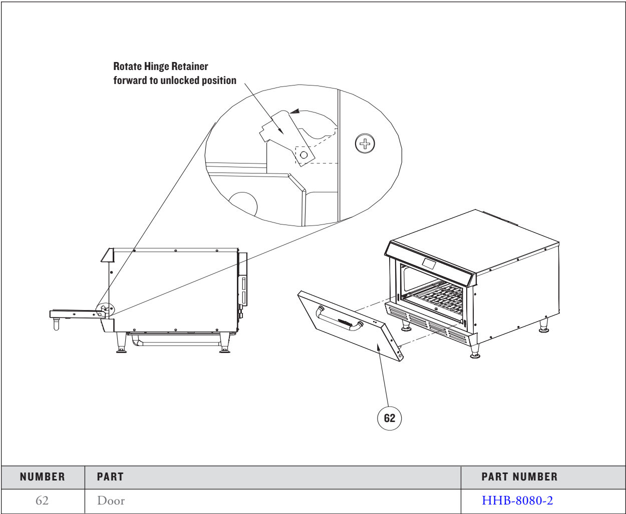
FIGURE 51: Removing the Oven Door
