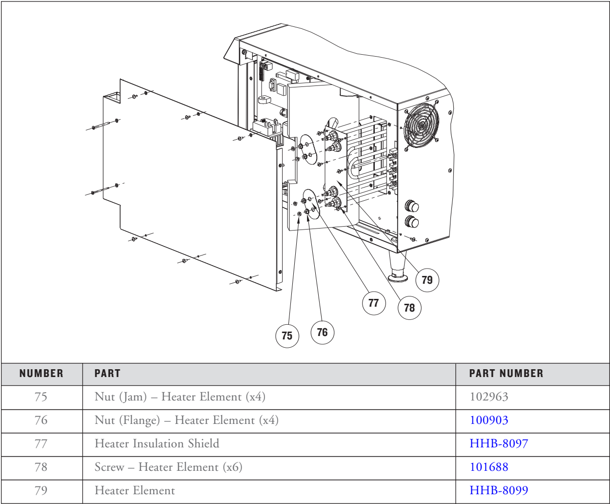
FIGURE 56: Removing the Heater Element
