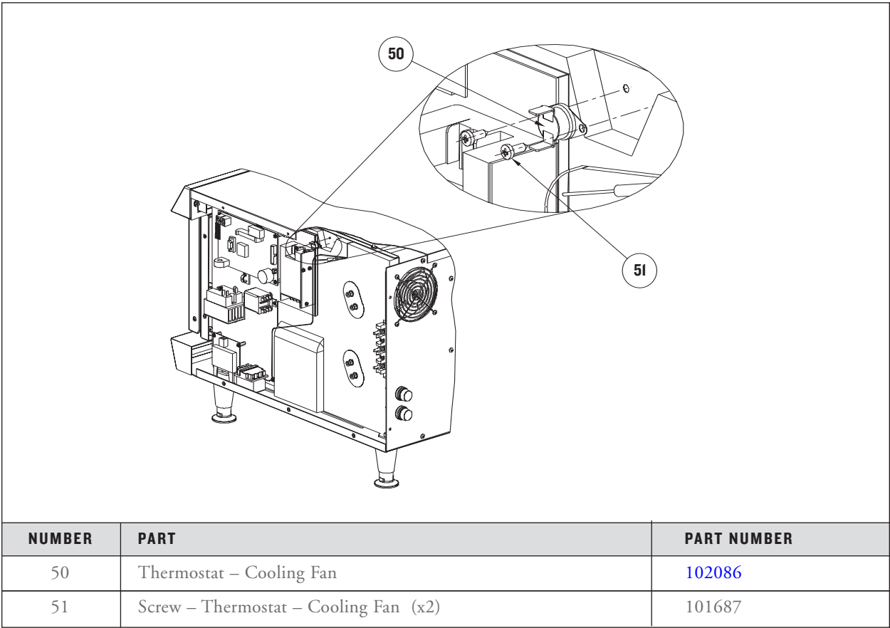
FIGURE 48: Removing Cooling Fan Thermostat
