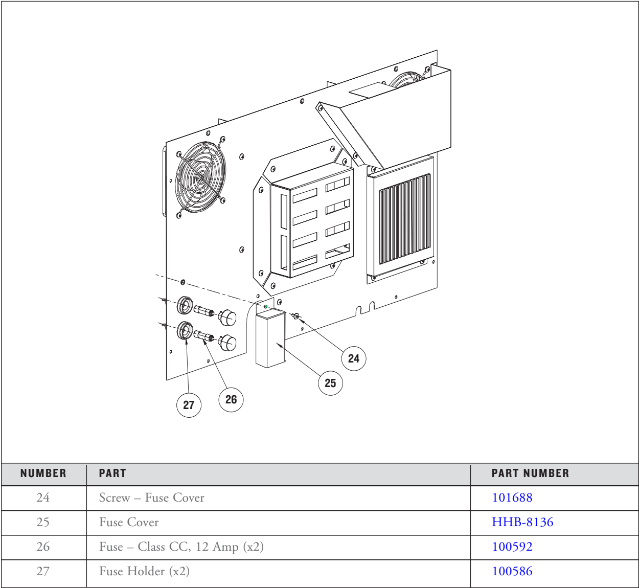
FIGURE 44: Removing Fuses
