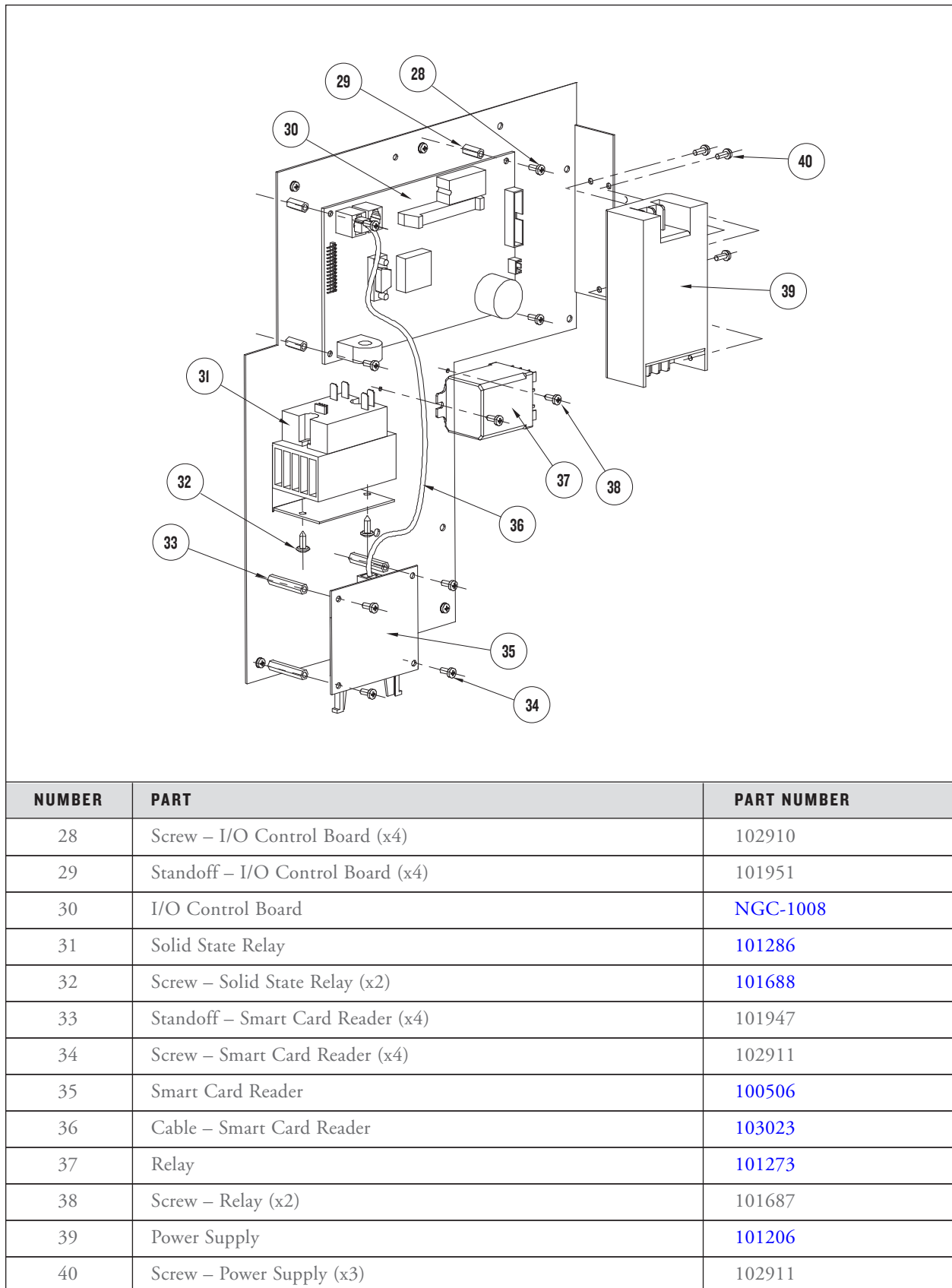
FIGURE 45: Component Plate Assembly
