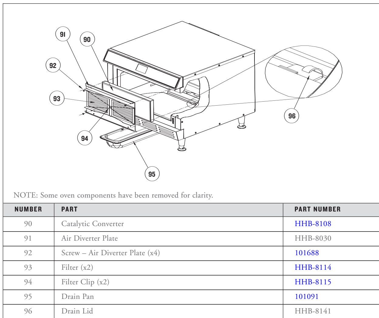
FIGURE 59: Filtering System Parts
