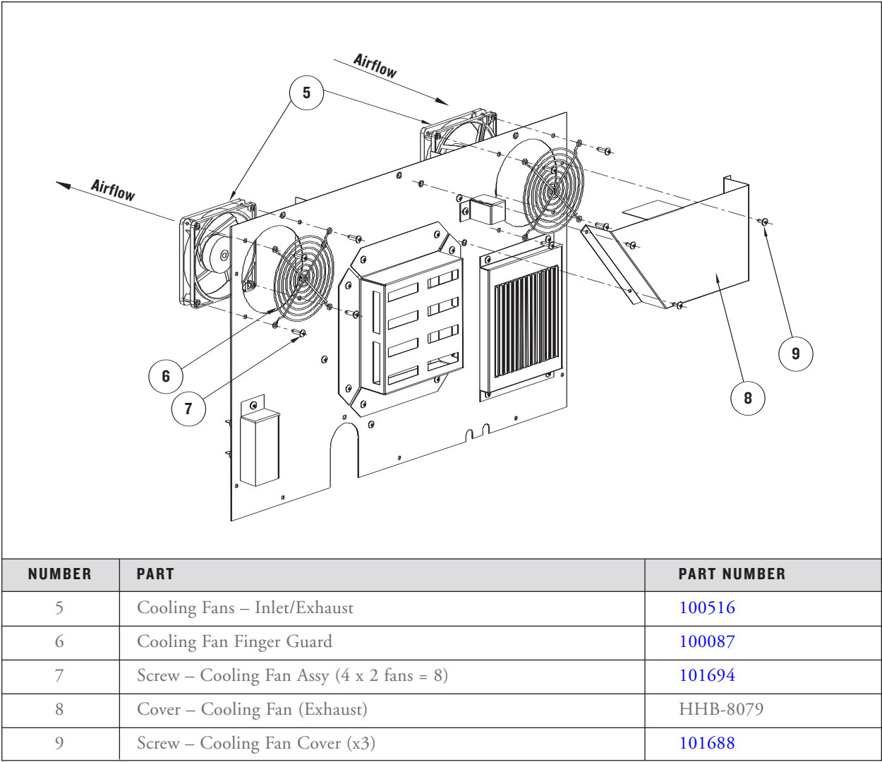
FIGURE 40: Replacing Cooling Fans
