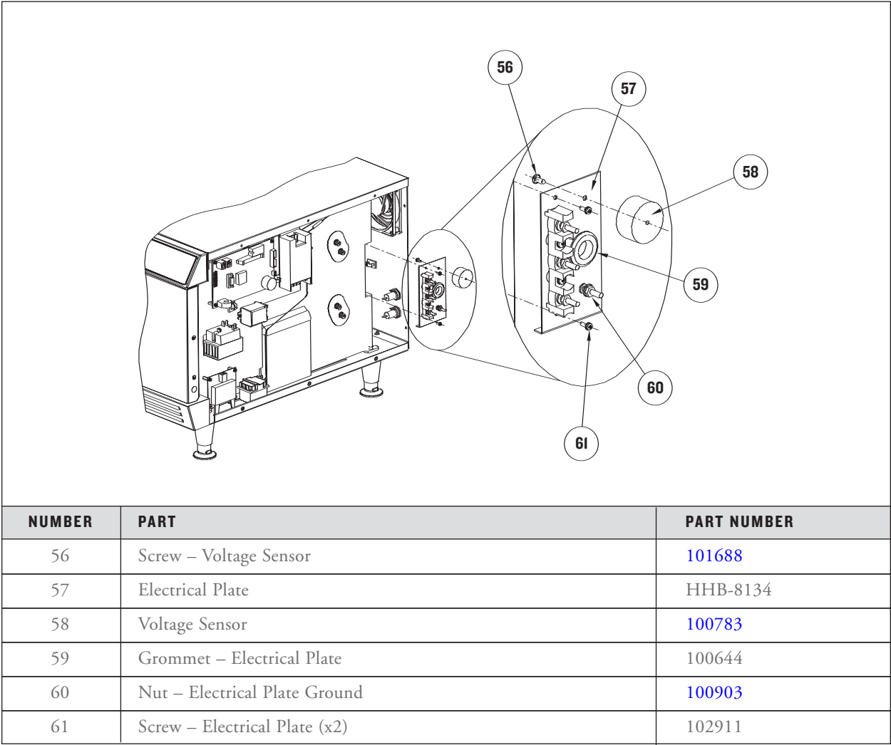
FIGURE 50: Replacing Voltage Sensor
