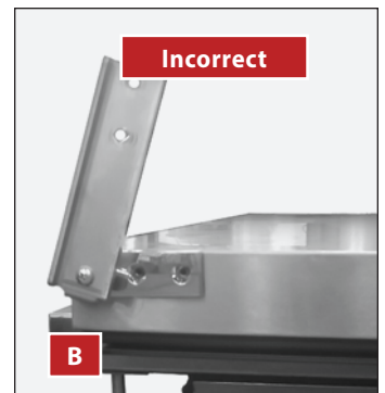
Fig. 7. Keep the washers in their original order.
