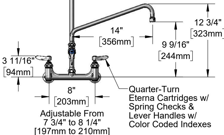
B-0107 1.15 GPM Spray Valve
