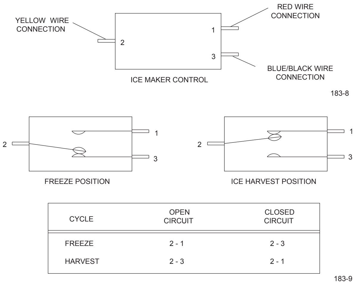
Figure 5. Temperature Controls - Manual Defrost Ice Makers
