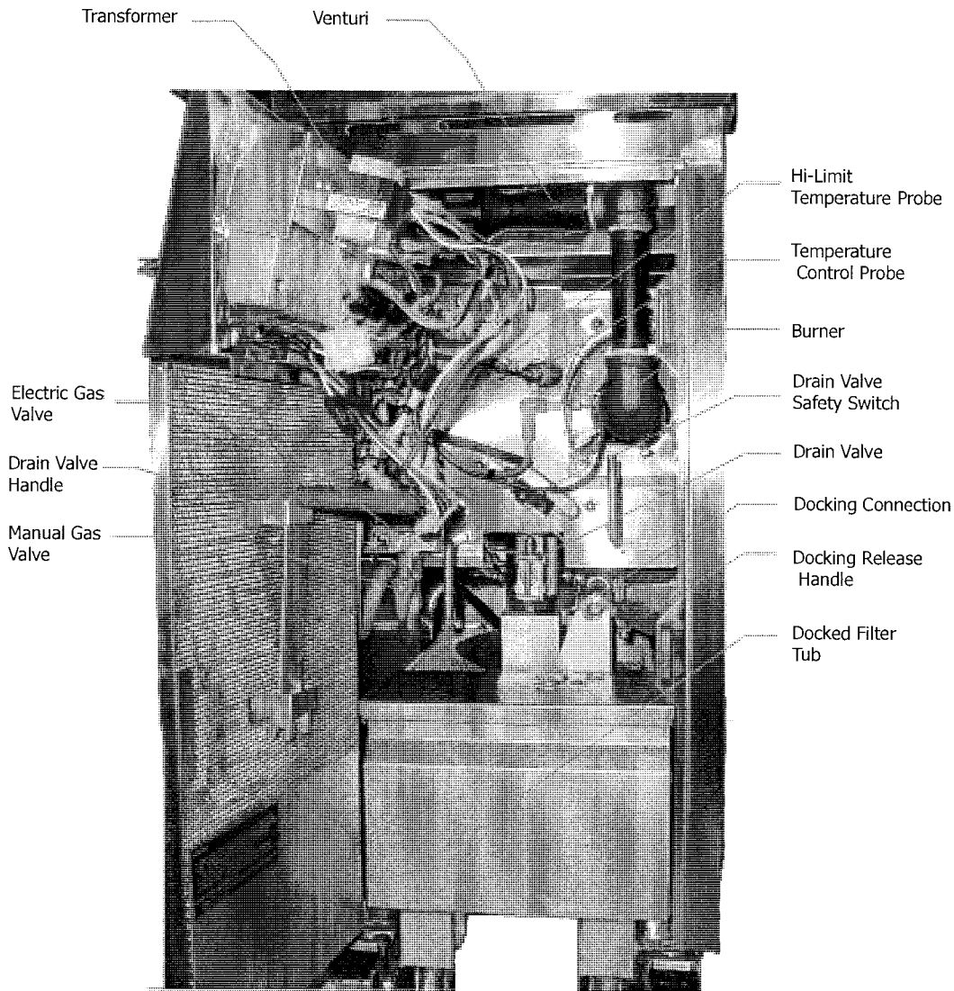
14" MODEL PAR-3-H GAS FRYER
