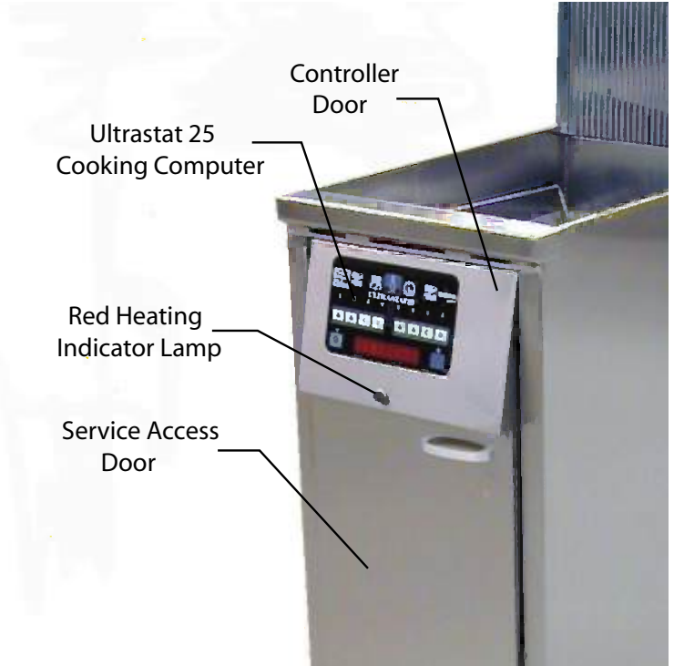
MODEL 14" PD GAS FRYER
