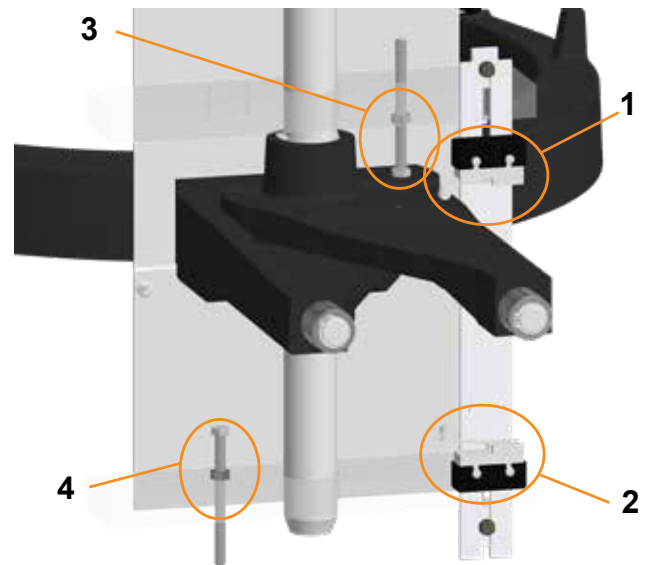
Fig. 8b Adjustment of bowl height (VL-1L, VL-1S):
