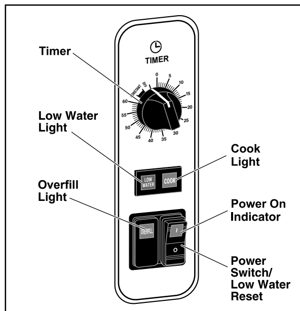
Figure 7: Controls
