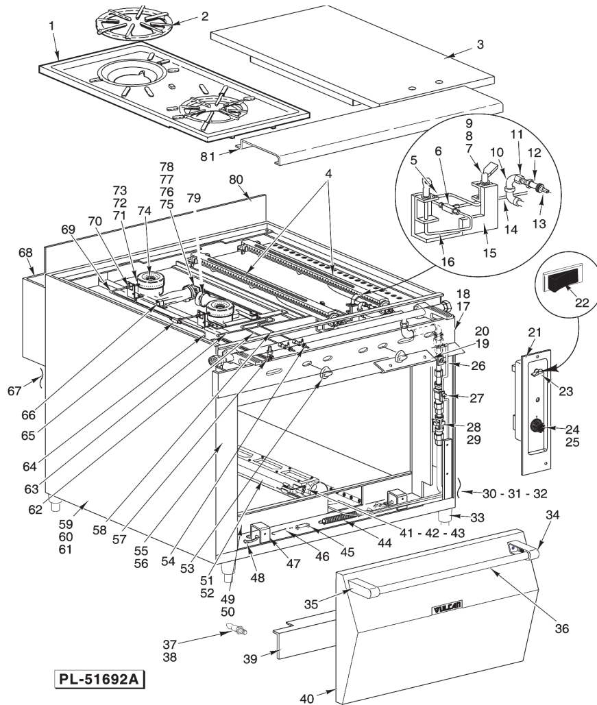
RANGE - GH45/72 &amp; GHM45/72
