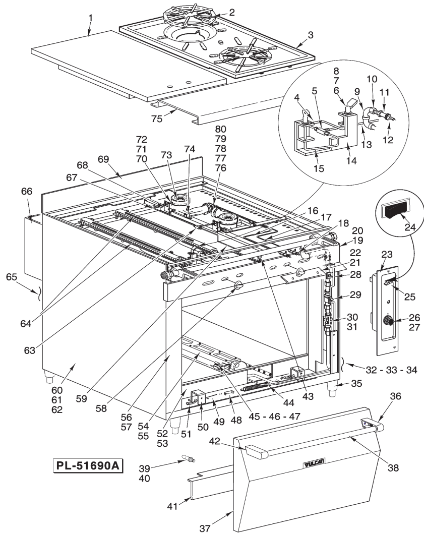
RANGE - GH72/45 &amp; GHM72/45
