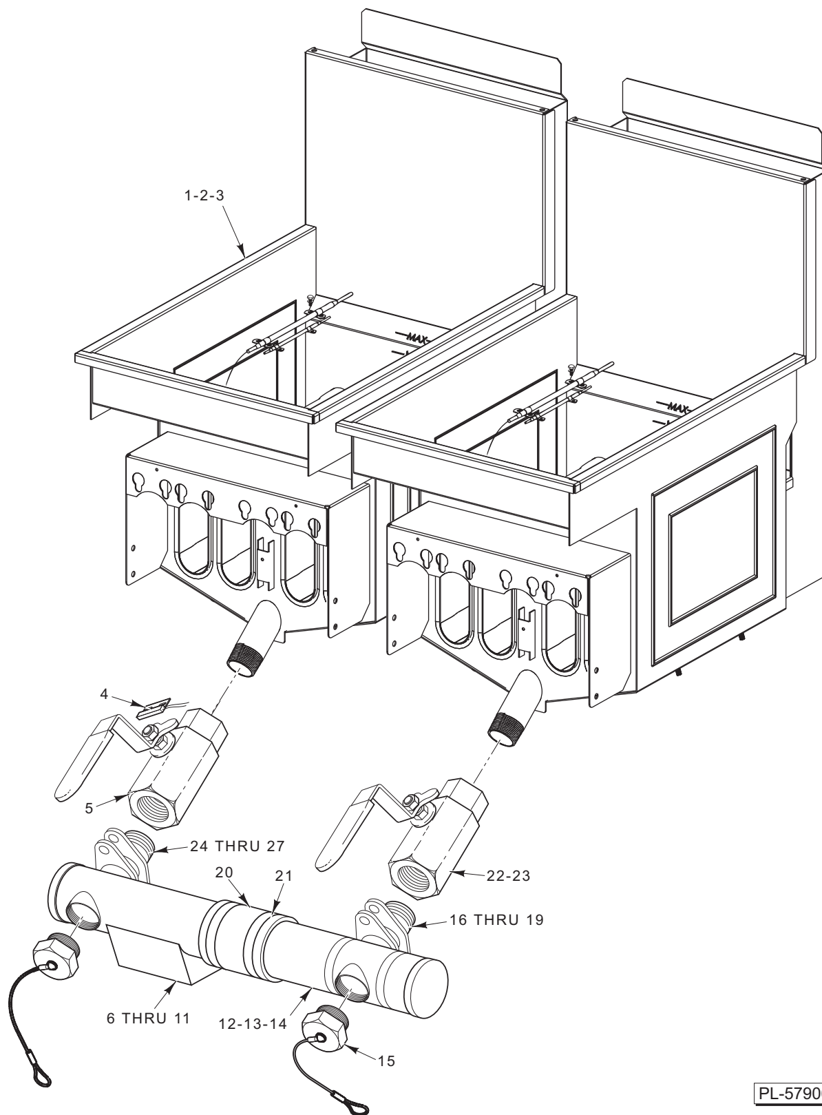
TANK AND DRAIN
