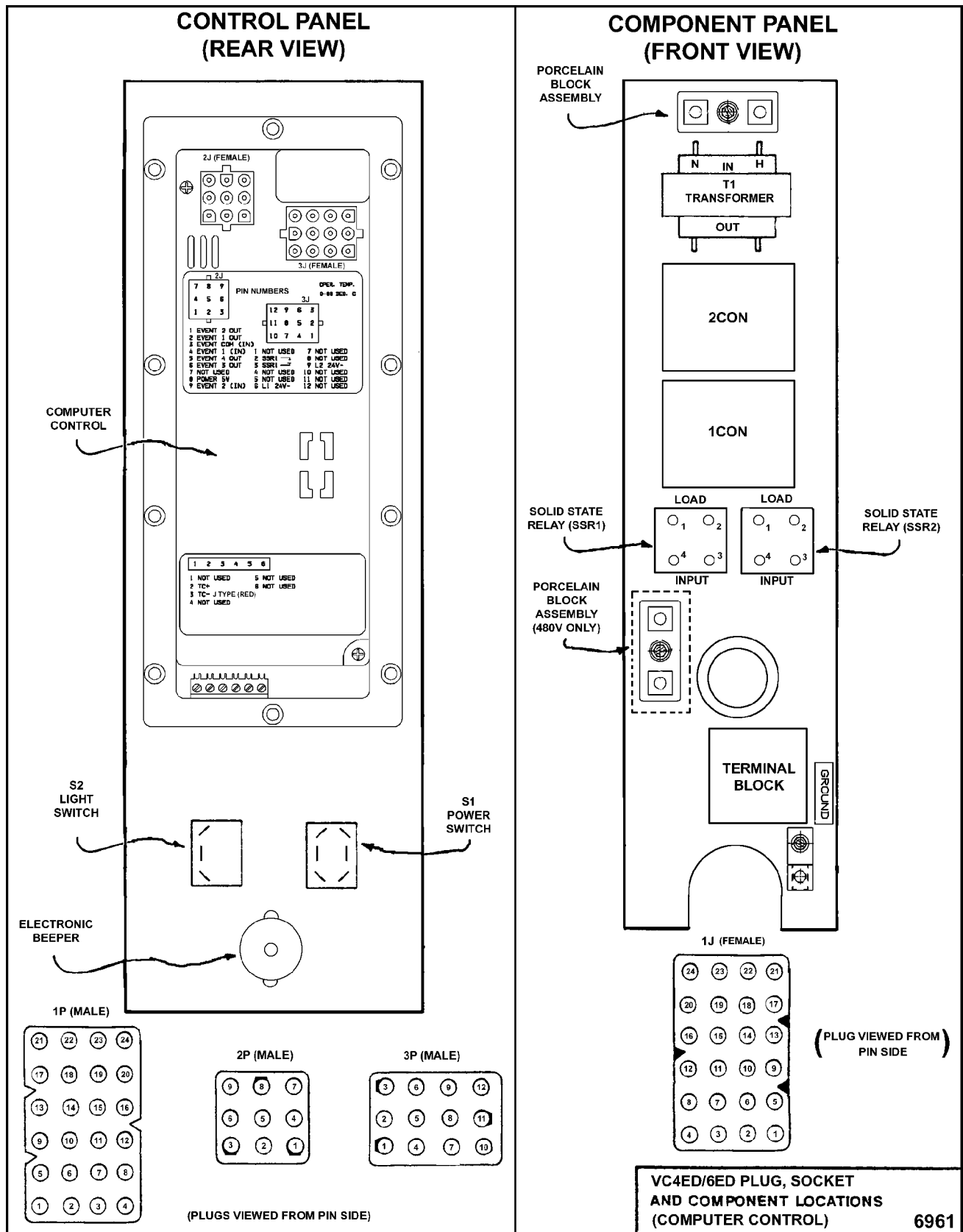
VC4EC/6EC - Plug, Socket and Components (Roast &amp; Hold Standard)
