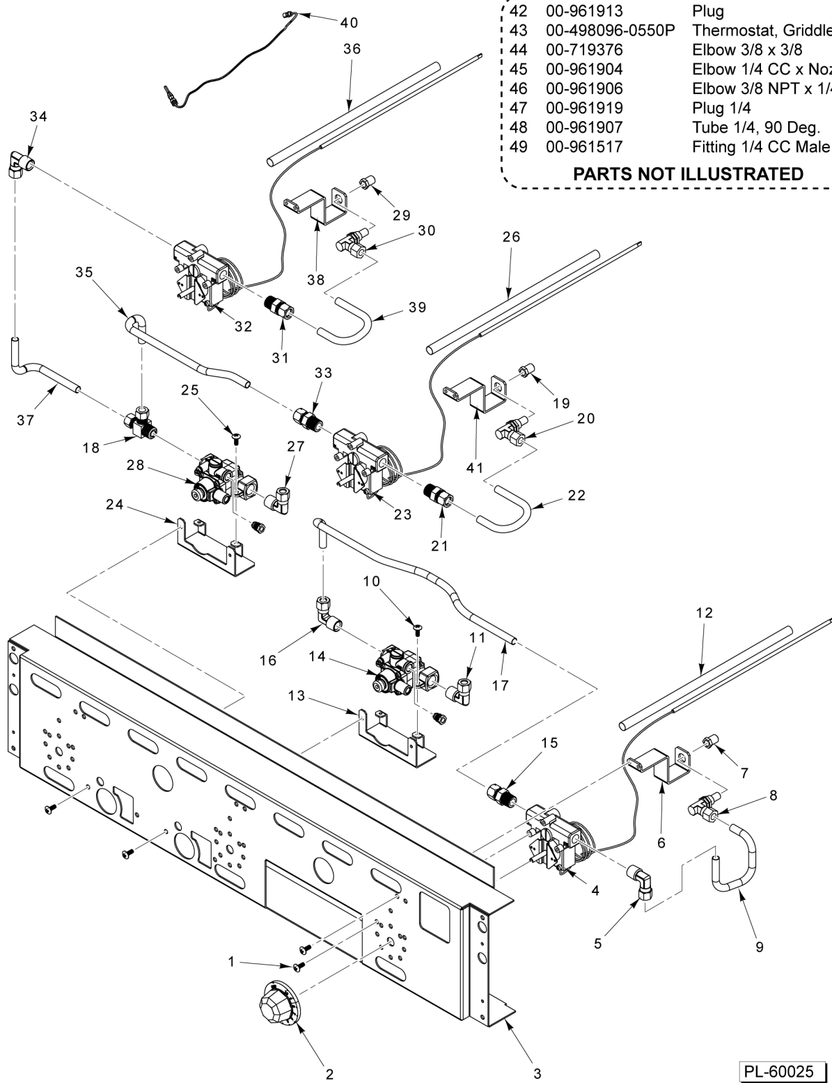
THERMOSTAT GRIDDLE CONTROL ASSEMBLY (36 INCH)
