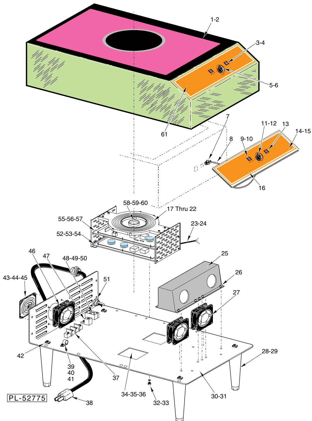
SINGLE INDUCTION COOKER
