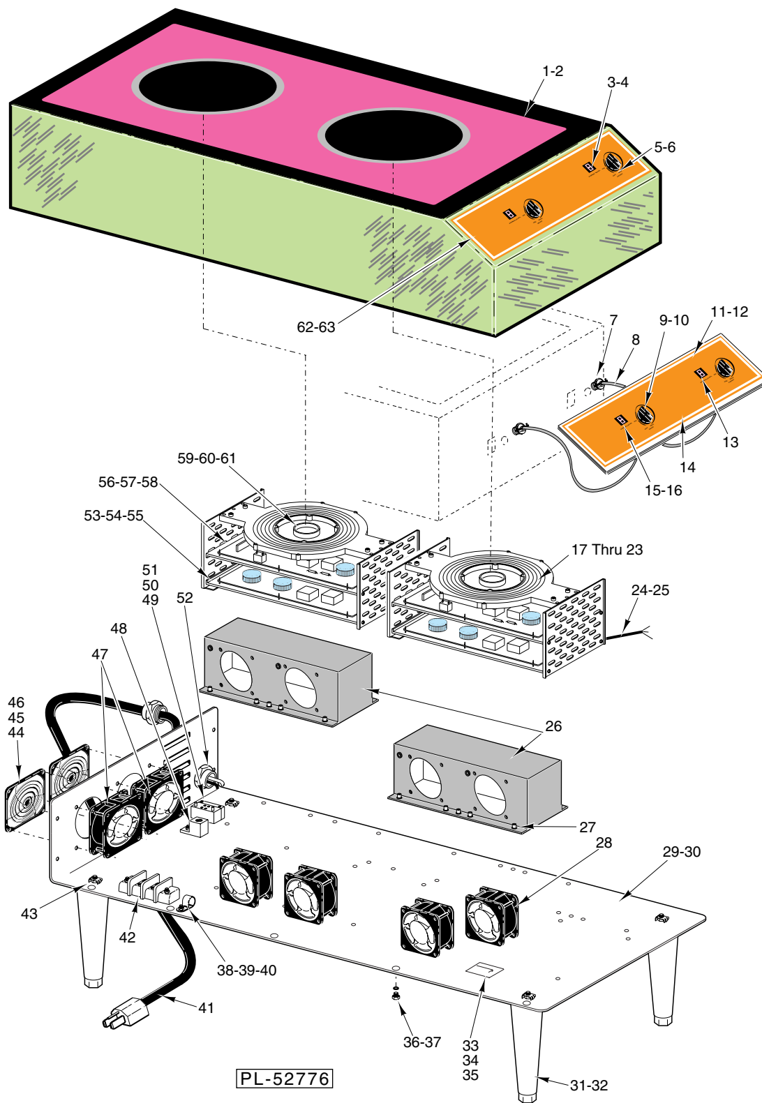
DOUBLE INDUCTION COOKER
